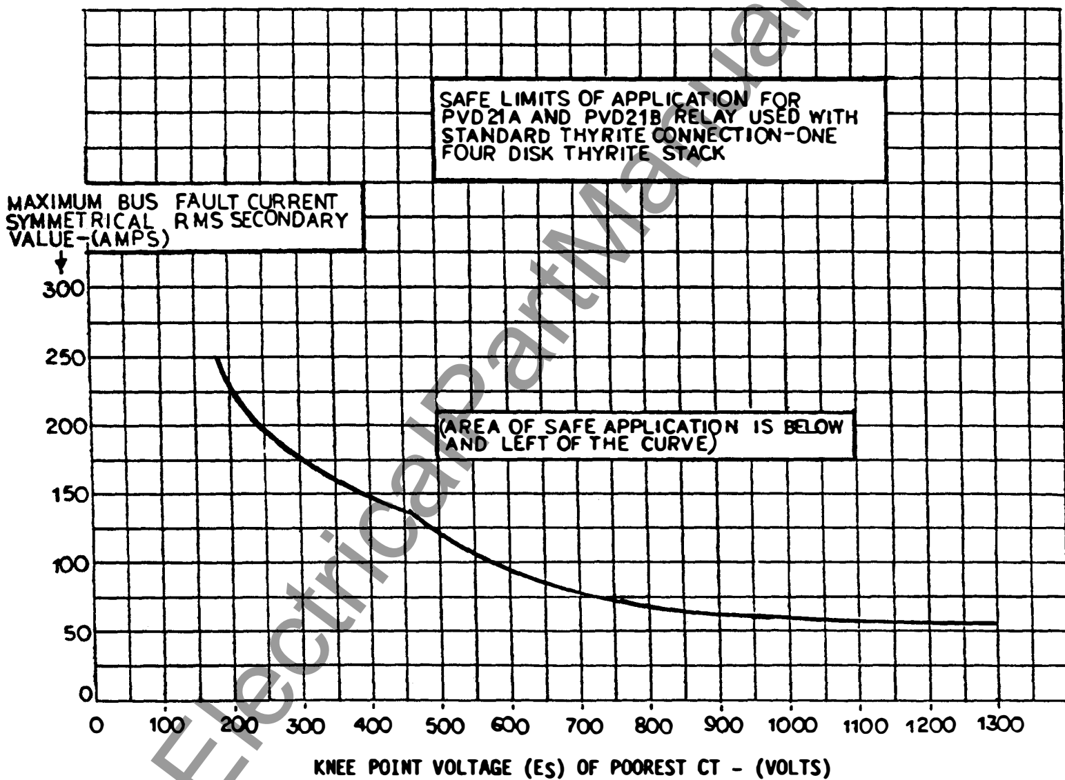
Figure 9 (0257A8588-2) Safe Application Limits for Type PVD21A or Type PVD21B Relays (One Thyrite® Stack)
