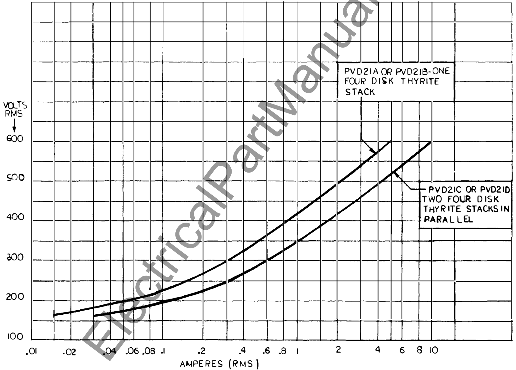
Figure 11 (0257A8589-1) Thyrite® Volt-Ampere Characteristics
