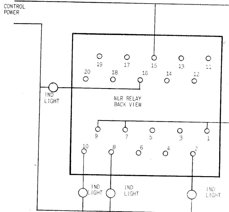
FIG. 10 (0178A9142-0) Test Connection For The NLR Type Relay
