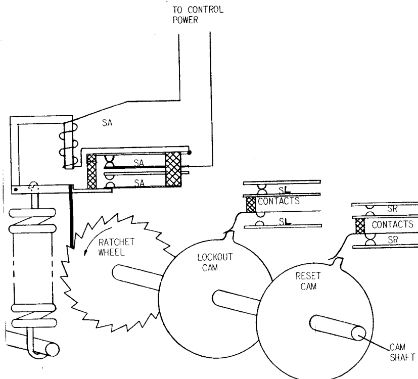
FIG. 9 (0178A9144-0) Stepping Switch For NLR Relay
