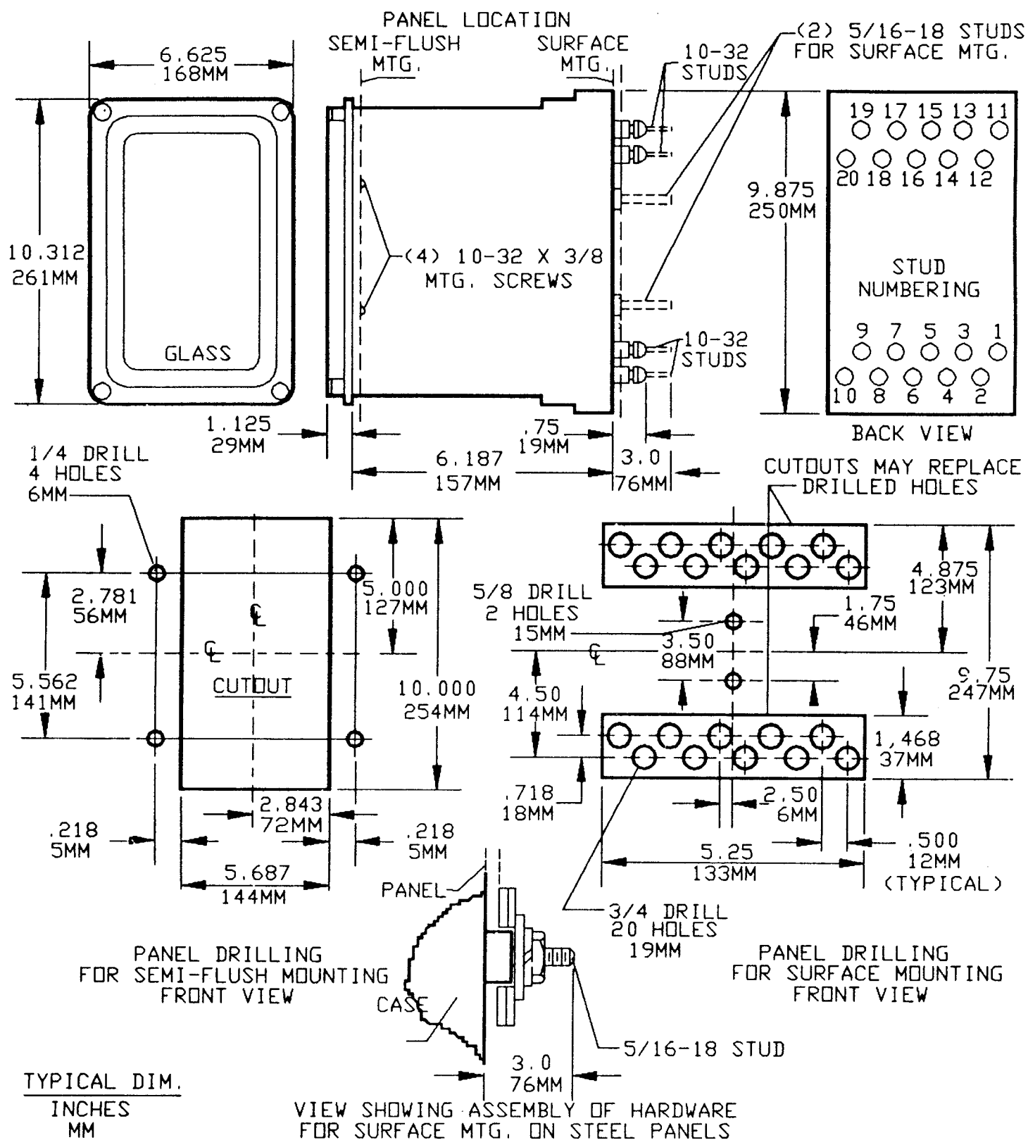
* FIG. 4 (K-6209272 [6]) Outline and Panel Drilling Diagram
