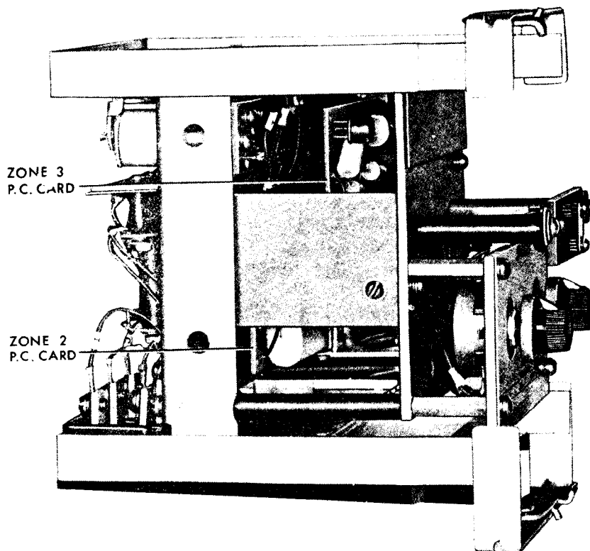
Figure 1A (8039885) Relay Type SAM16A12A Removed from Case (Front View)
