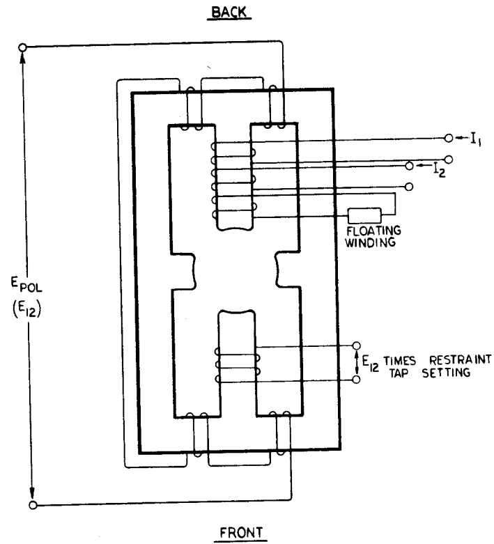
Fig. 5 (0208A5577-0) Schematic Connections of Typical M2 Unit
