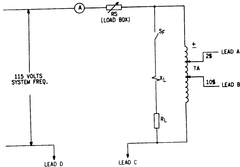
Fig. 11 (0195A4991-1) Test Connections for Checking the Correct MHO Unit Operation
