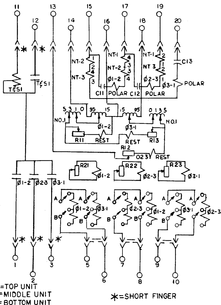
* Fig. 10 (0178A7133[5]) Internal Connections Diagram for the CEY52A Relay (Front View)
