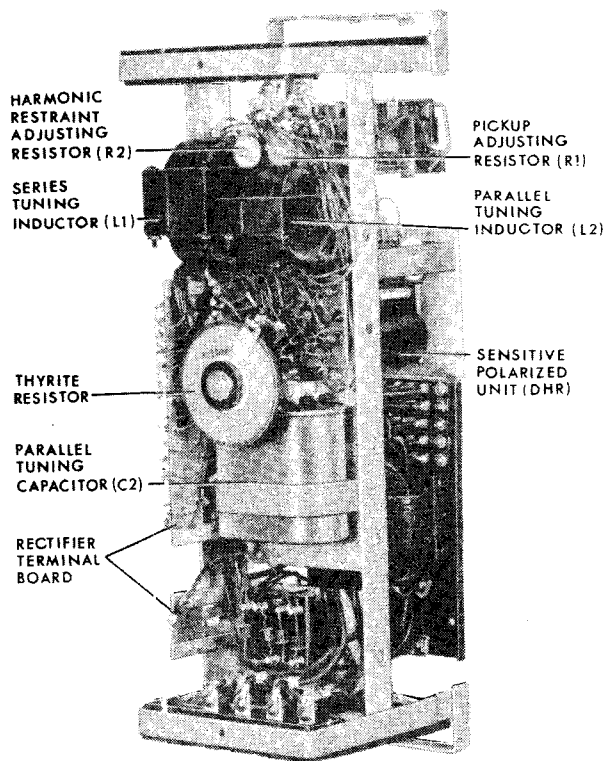
Fig. 1B (8035510) Type BDD17B Relay, Cradle Removed From Case, Rear View.
