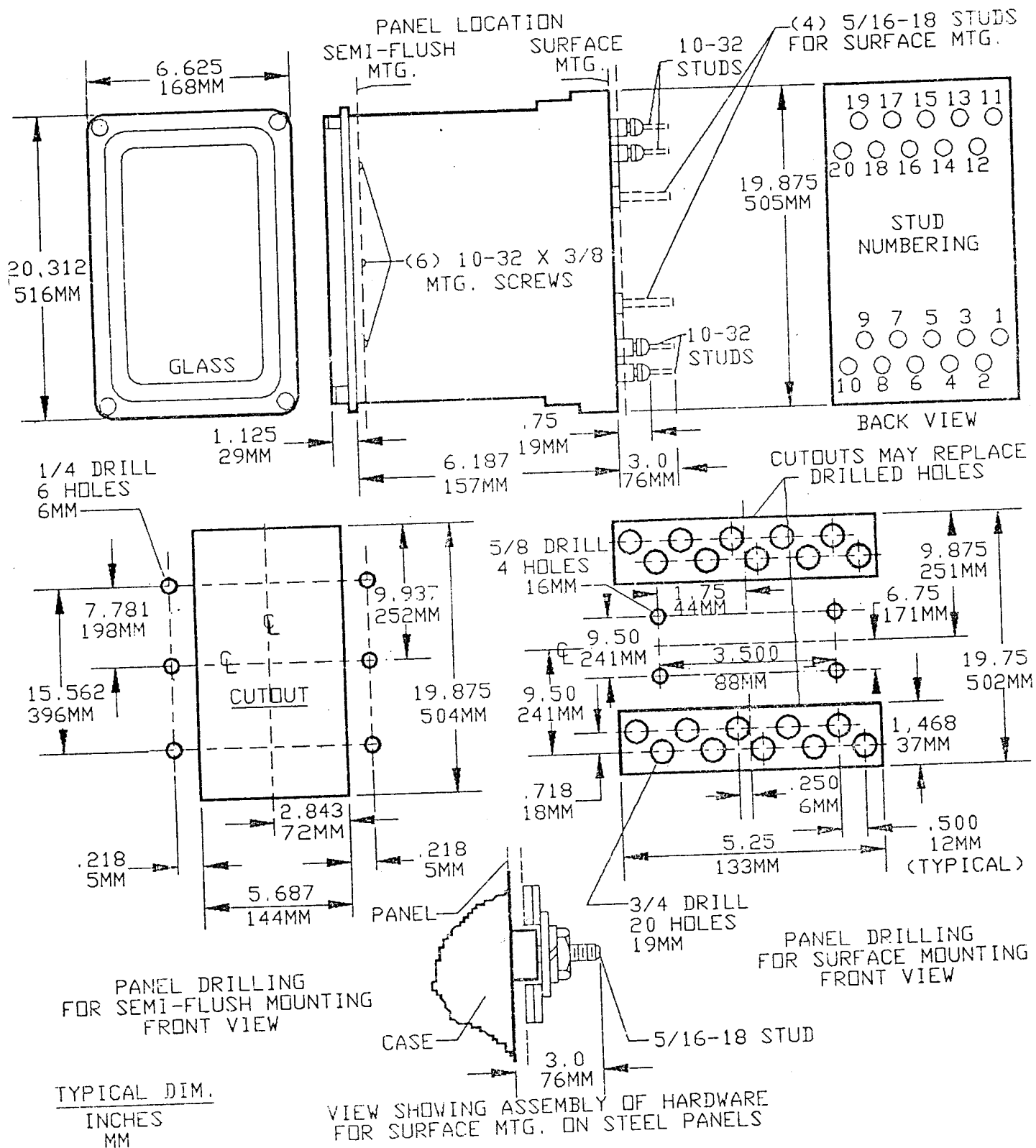
Fig. 5 (6029276 [5]) Outline and Panel Drilling Dimensions for Relay Type BDD17B.
