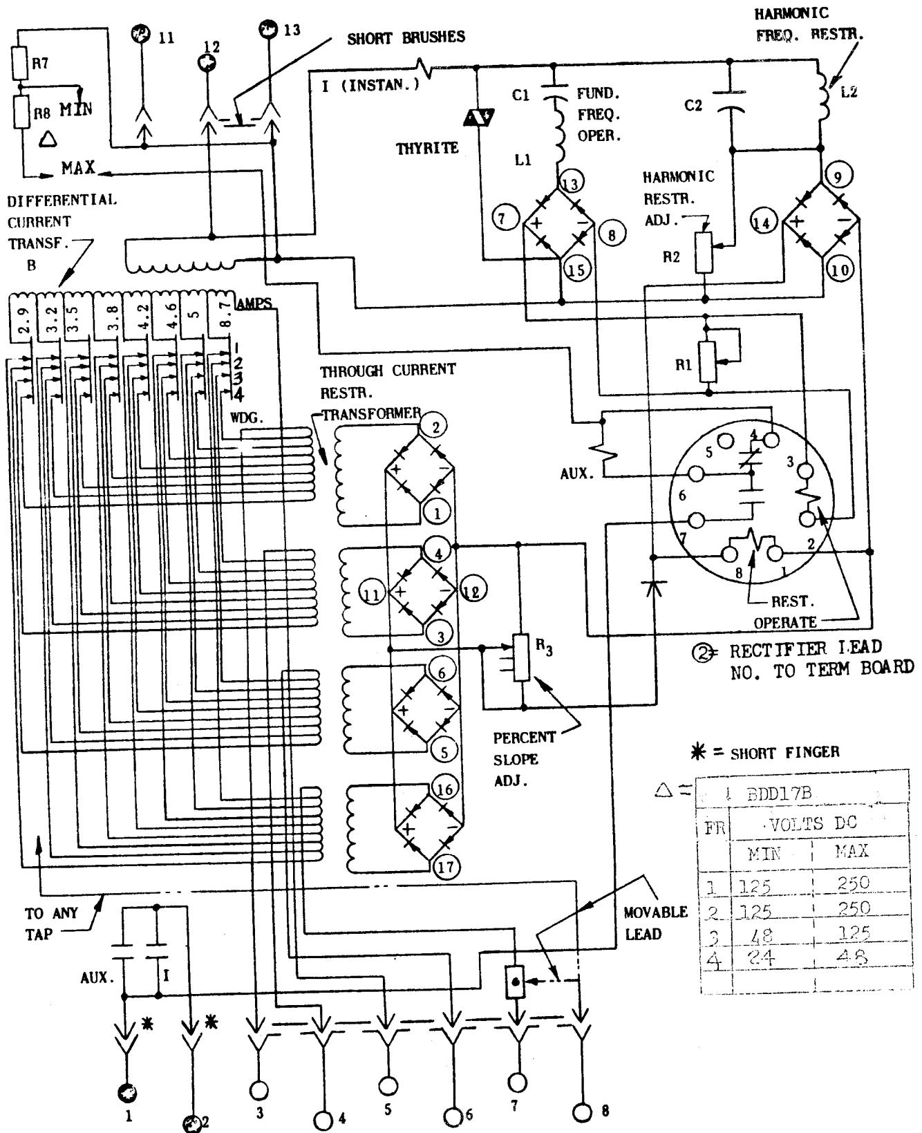
Fig. 2 (Q178A9048 [2]) Internal Connections for Relay Type BDD17B.
