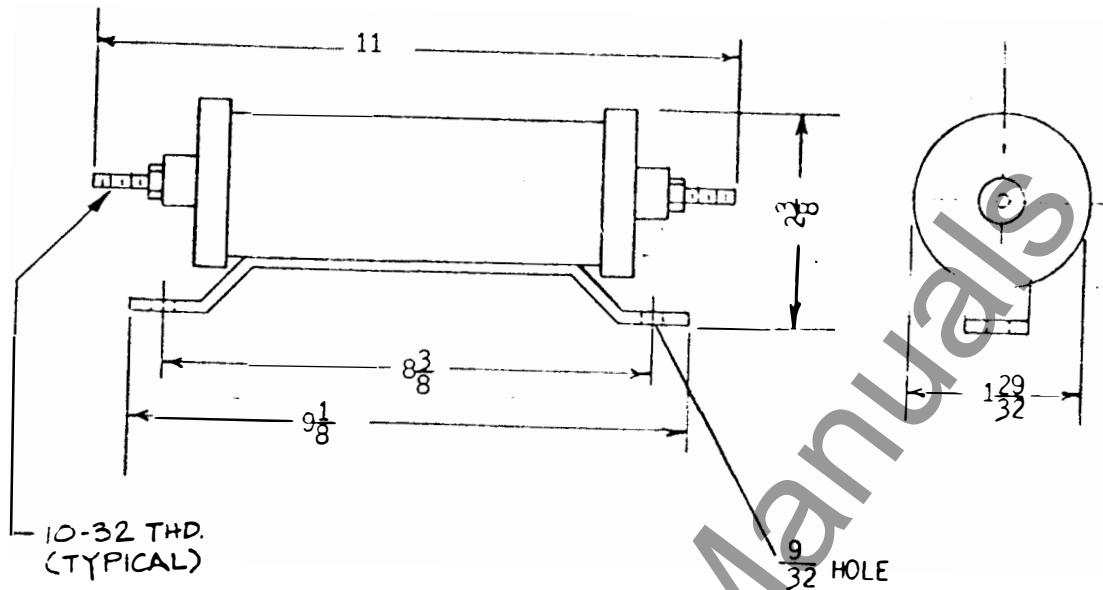
* Fig. 4 Outline of External Resistor used with Forms 25 and 26 of these Relays
