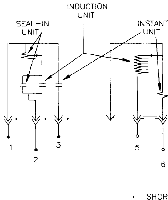
Fig. 12. (K-6209661 [11]) Internal Connections for the Type IAC51B Relay (Front View)
