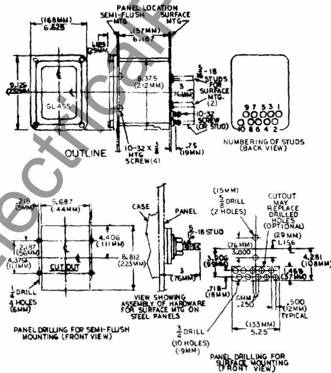
* Figure 6. (6209271-6) Outline and Panel Drilling for the Type IAC59A Relay
