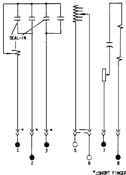
Fig. 5 Internal Connections (Front View) of ICW52B Relay
