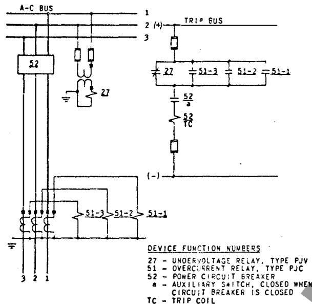
Fig. 4 Elementary Connections Of Circuit Protected Against Overcurrent And Undervoltage
