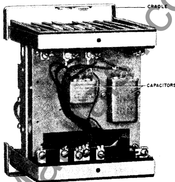
Figure 11 (8014331) Type ICR53A Relay, Unit in Cradle (Rear View)
