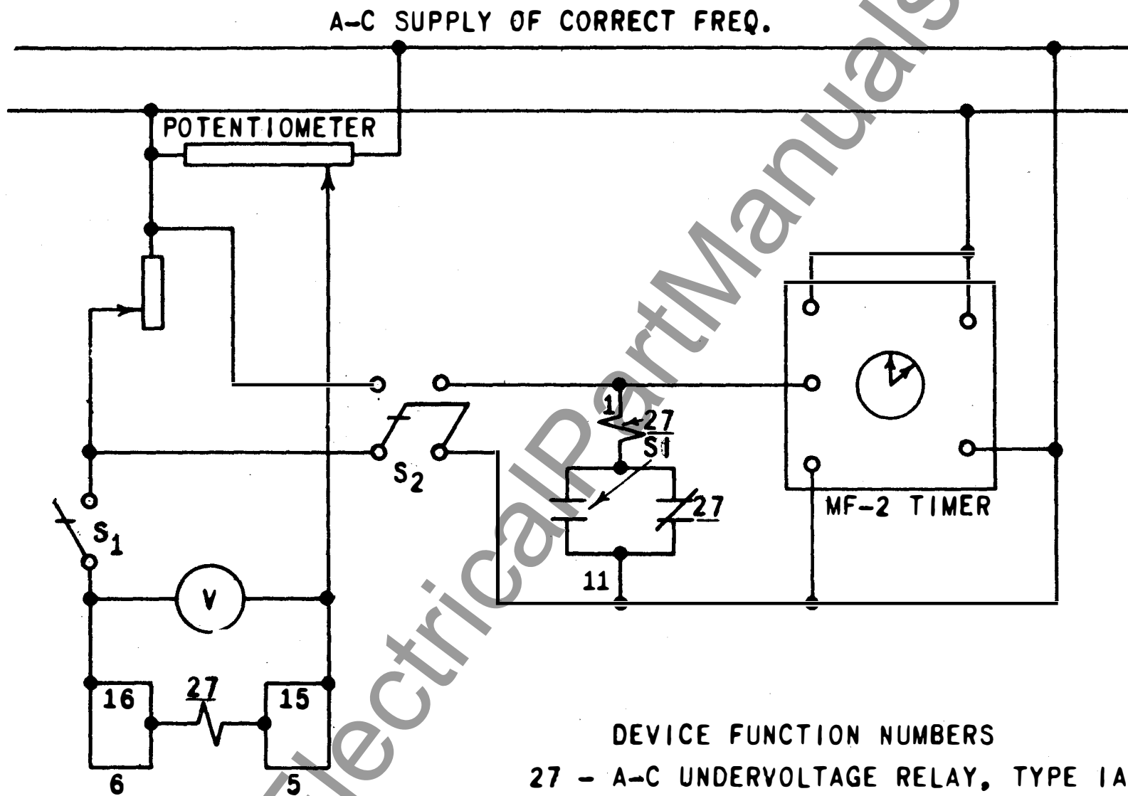
Figure 9 (6154392-5) Connections for Testing Types IAV54 and IAV55 Relays
