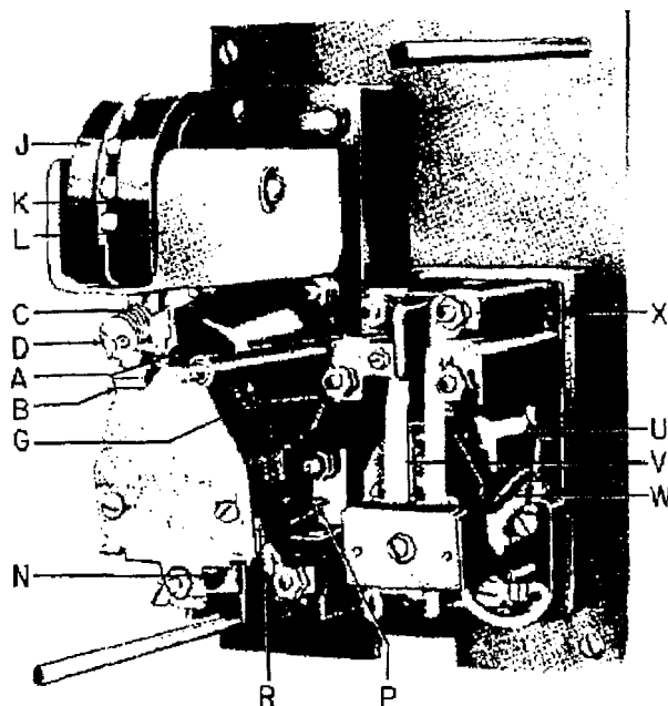
Fig. 1. Type HKA relay, moderate duty, using HGA style auxiliary unit, side-by-side arrangement
