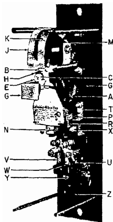
Fig. 3. Type HKA relay, heavy duty, using HMA style auxiliary unit, and vertical arrangement
