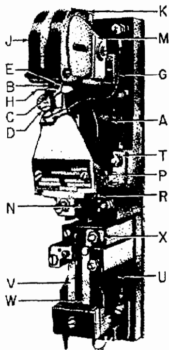
Fig. 2. Type HKA relay, light duty, using HGA style auxiliary unit and vertical arrangement
