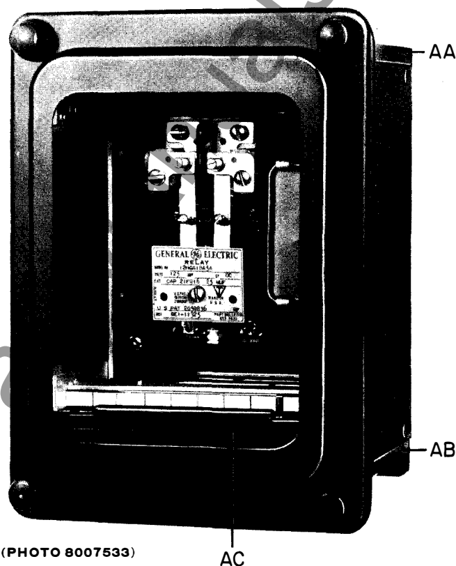
Fig. 2. Type HGA18 reclosing relay (typical of relays in drawout "A" case)
