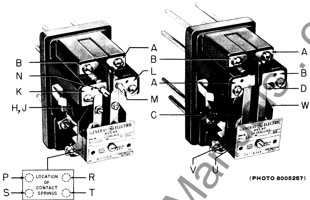
Fig. 3. Type HGA14 relay (cover removed)
