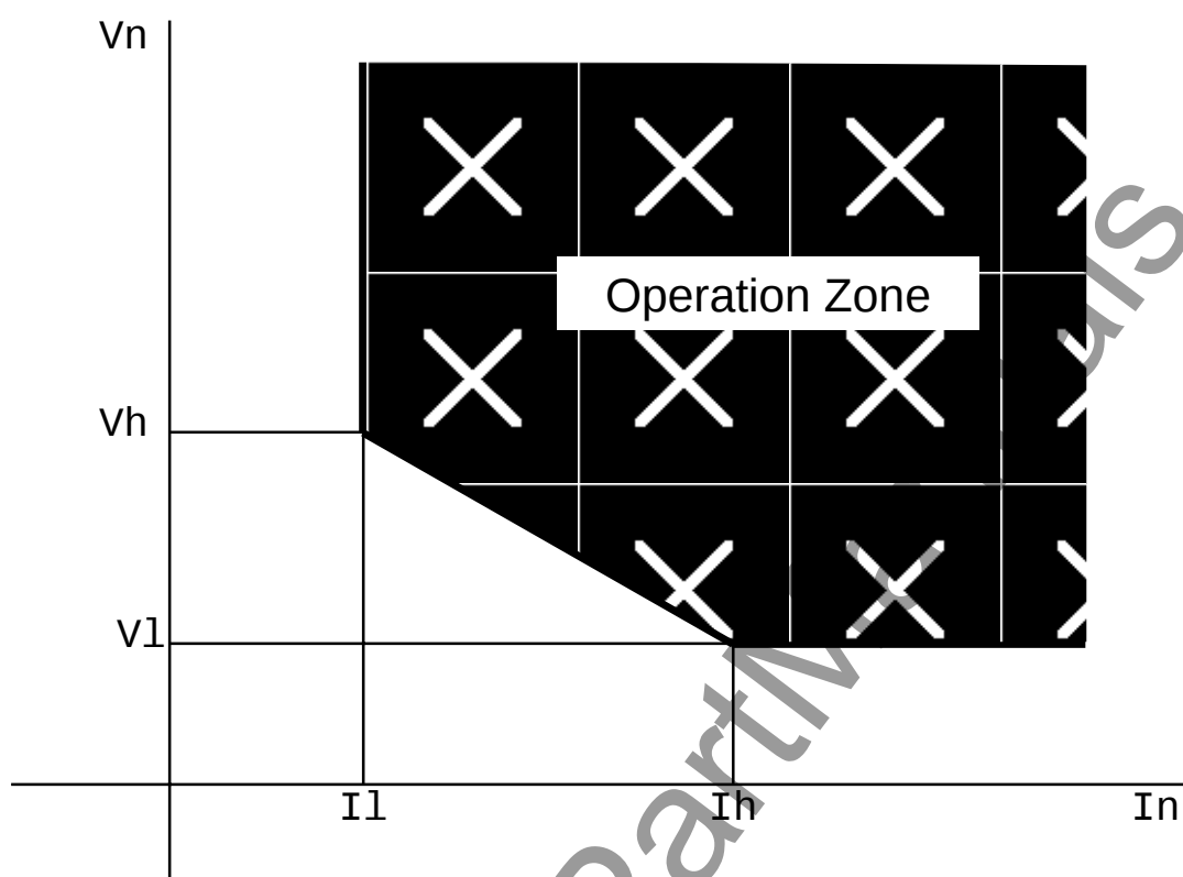
Figure A1 V-I Relation in 67N unit
