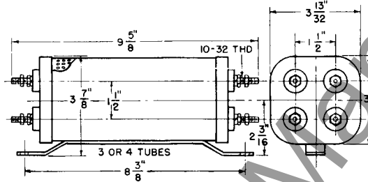
Fig. 12. Four-tube, Form-3 resistor.
