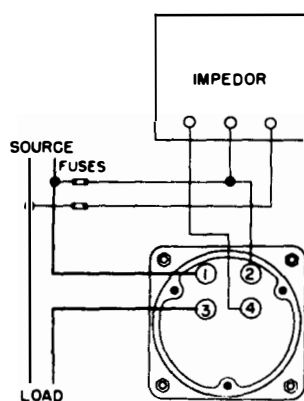
Without transformers
