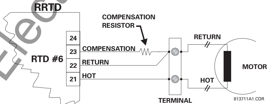
Figure 6-2: 2 WIRE RTD LEAD COMPENSATION
