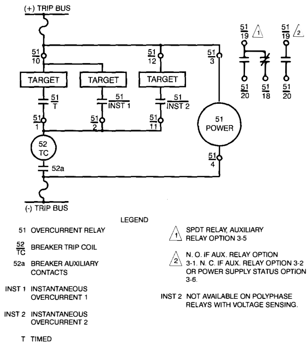
Figure 4 - Control Circuits
