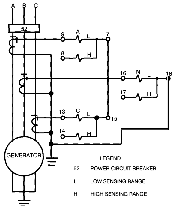
Figure 7 - Two-Phase-and-Neutral Current Sensing
