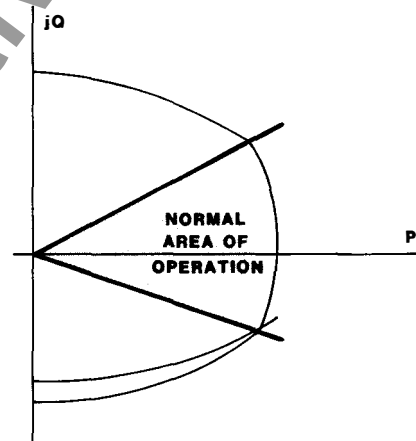
FIGURE 3. NORMAL AREA OF GENERATOR OPERATION
