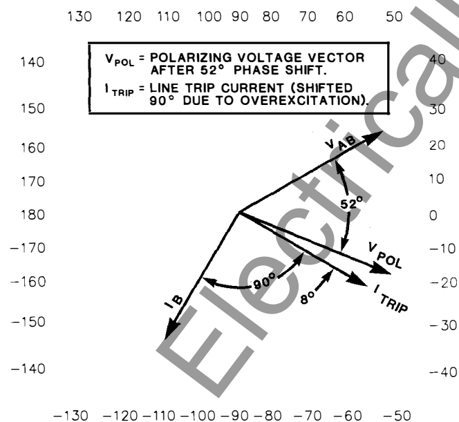
FIGURE 6. PHASE SHIFT EXAMPLE
