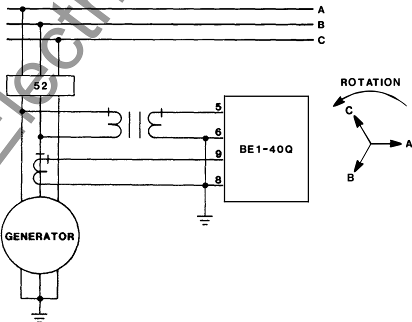
FIGURE 9. RECOMMENDED SENSING CONNECTIONS
