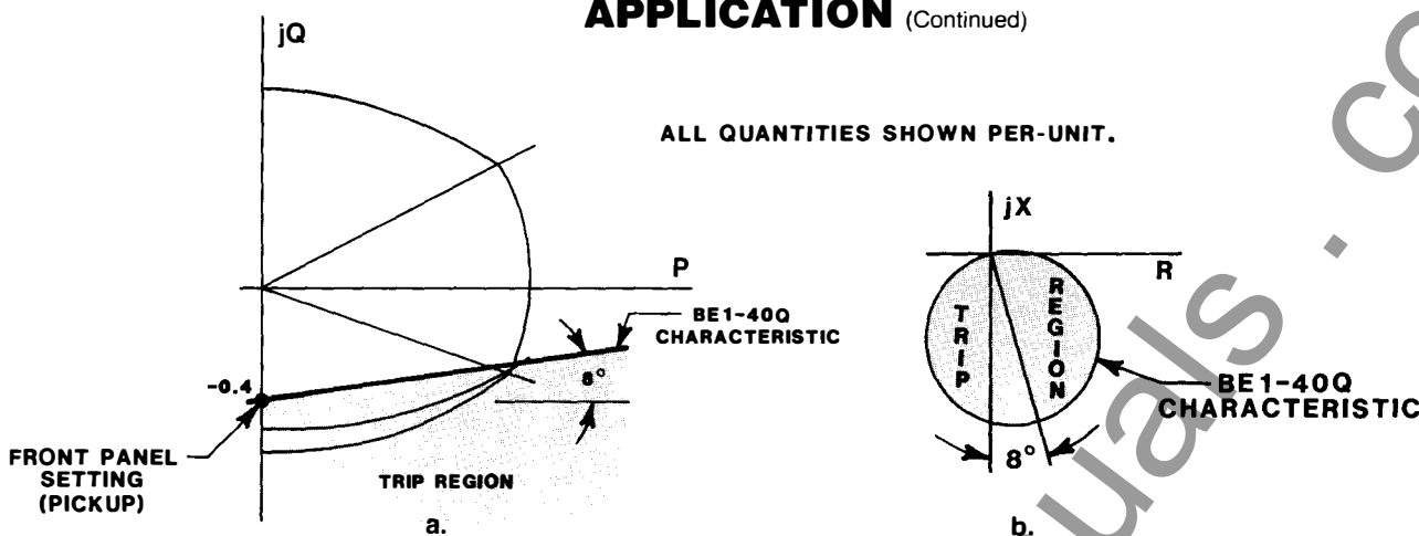
FIGURE 4. BE1-40Q OPERATING CHARACTERISTIC
