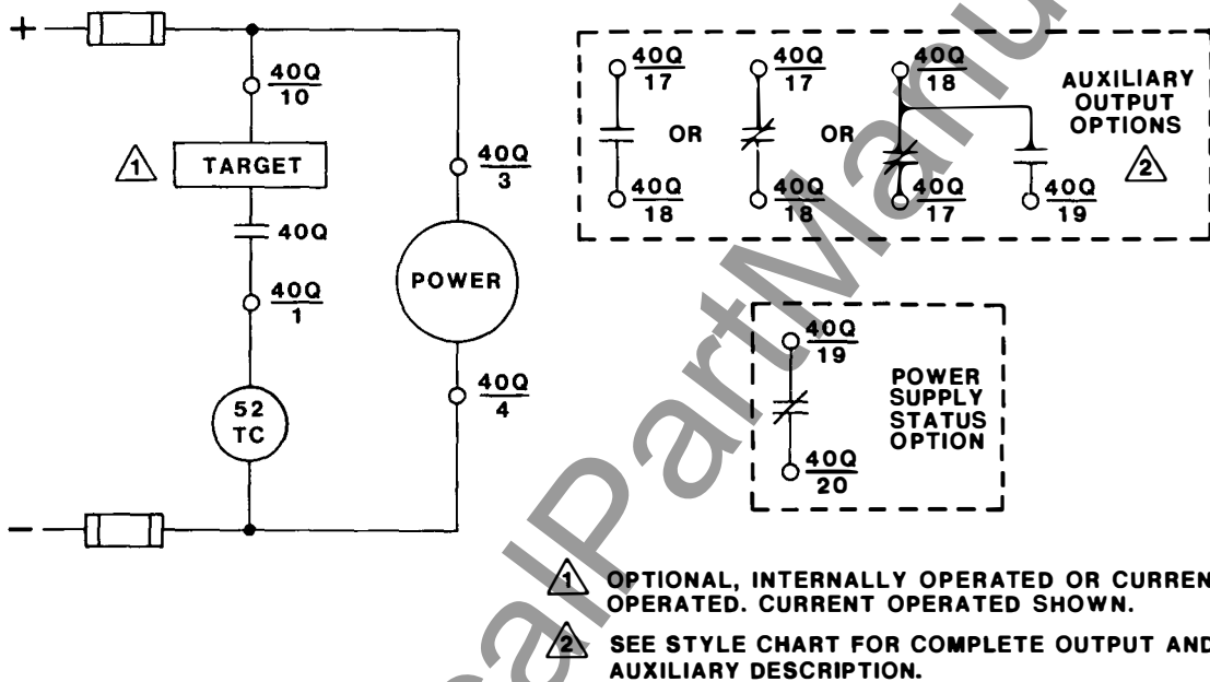
FIGURE 8. OUTPUT CONNECTIONS
