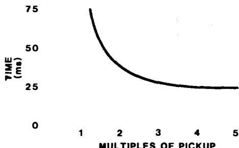
FIGURE 7. INTEGRATOR STEP RESPONSE OF TRANSDUCER
