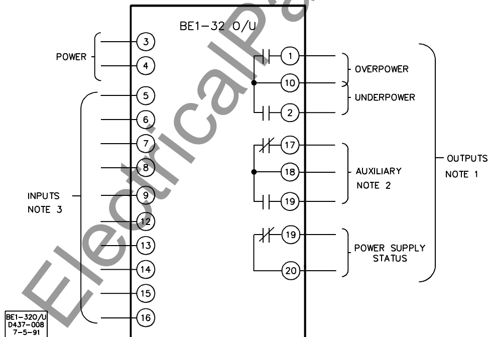
Figure 4-23. BE1-32 O/U Typical External Connections
