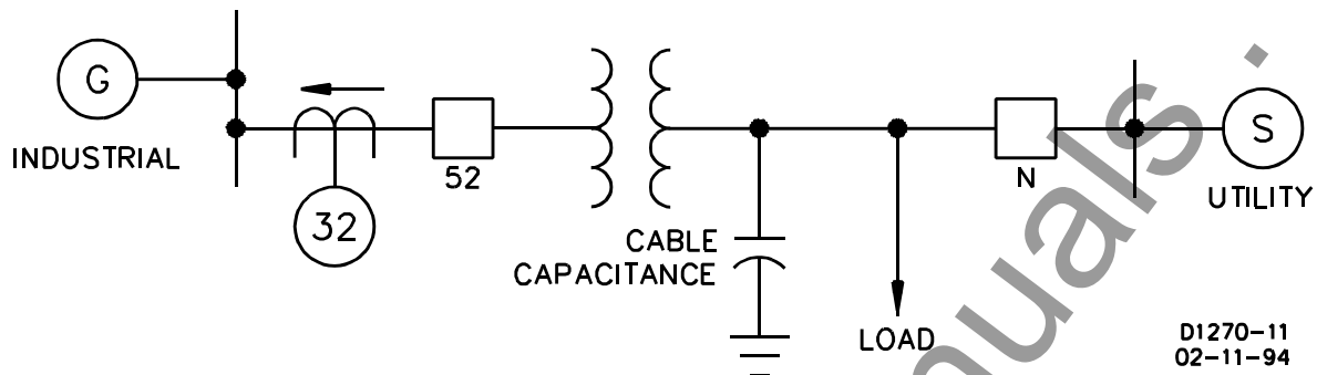
Figure 1-6. Breaker Opening Detection
