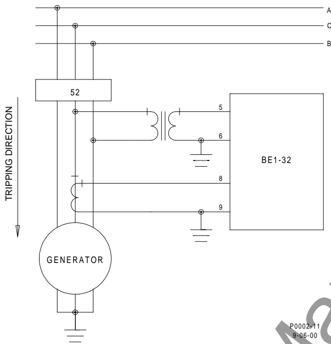
Figure 4-26. Type B or V Sensing with ACB Rotation
