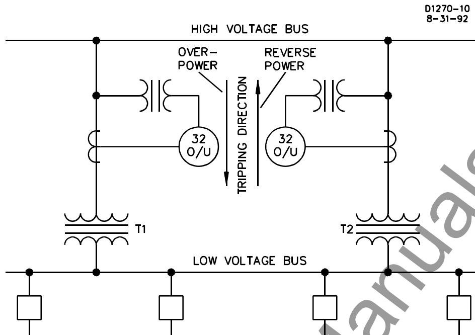
Figure 1-4. Power Relay Distribution Protection
