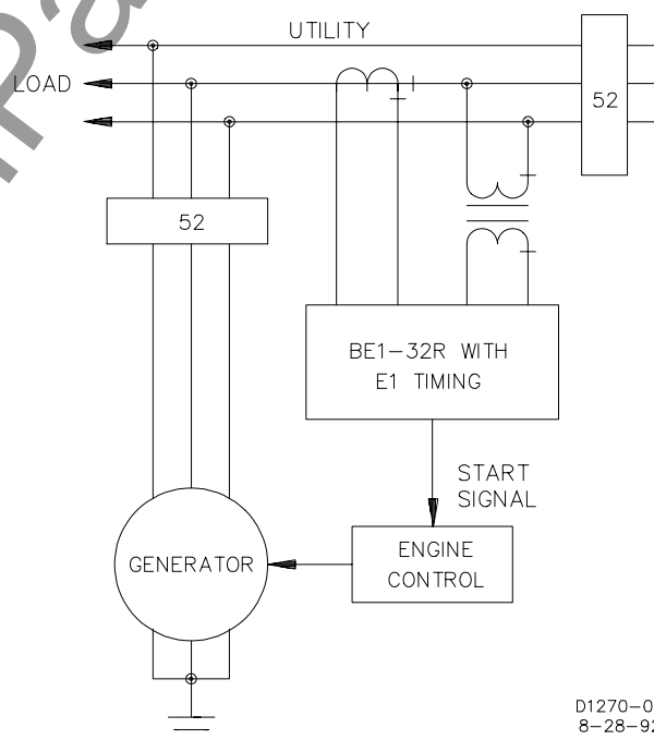
Figure 1-2. Power Relay Start Control
