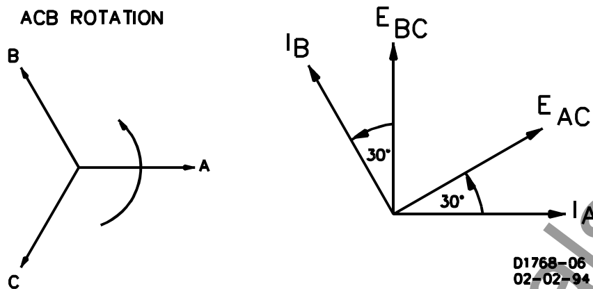
Figure 3-3. Type E Sensing With ACB Rotation
