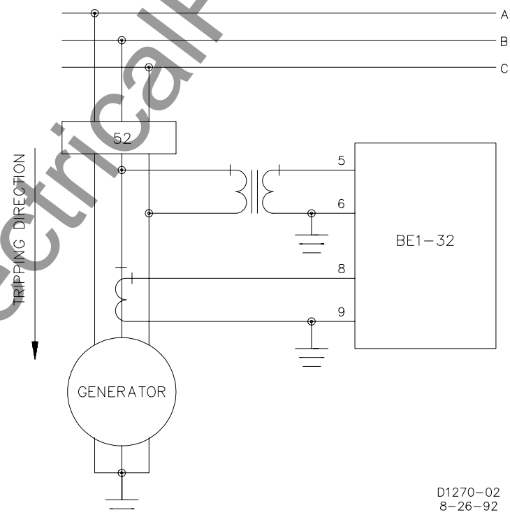
Figure 4-25. Type B or V Sensing With ABC Rotation
