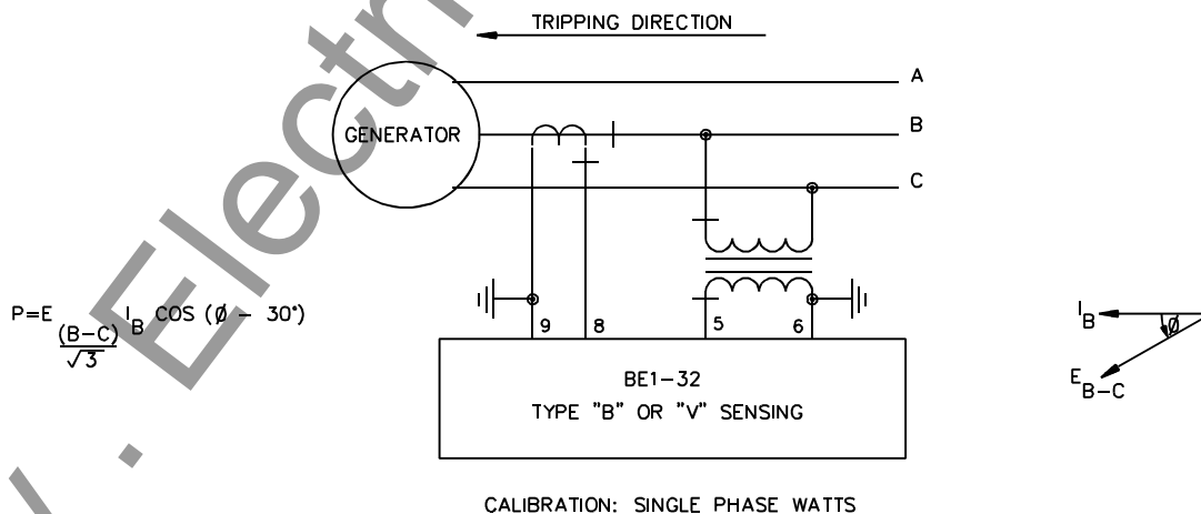
Figure 3-7. Type B or V Sensing
