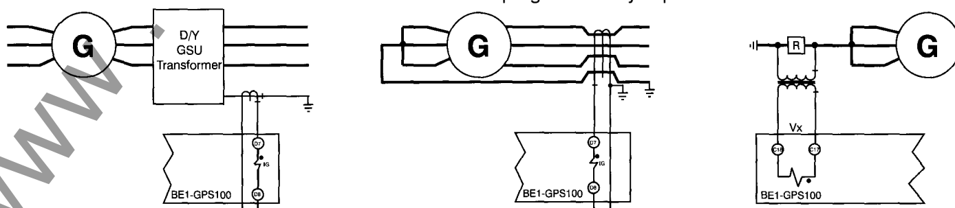
Figure 2A - Typical Alternate Connections for Vx and IG
