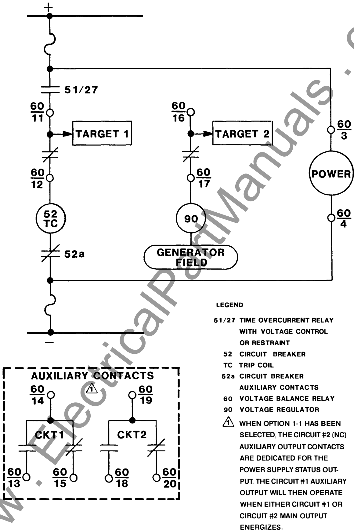
FIGURE 4. CONTROL CIRCUITS
