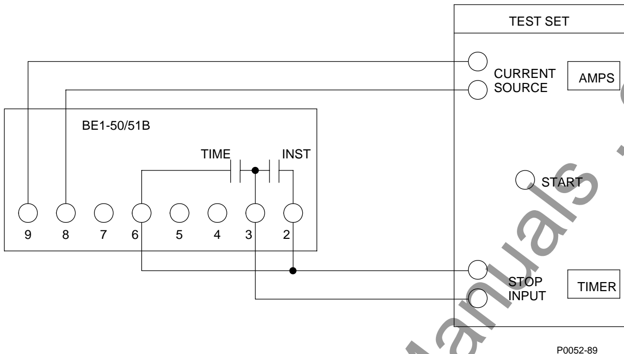
Figure 5-1. Pickup and Timing Test Setup
