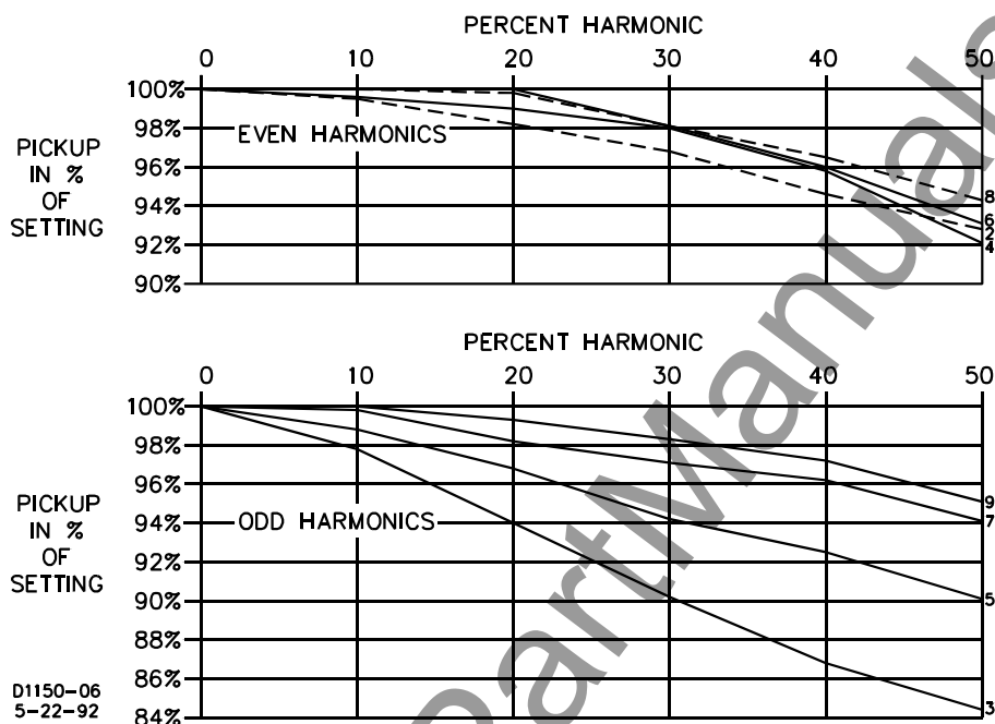
Figure 1-4. Harmonic Response
