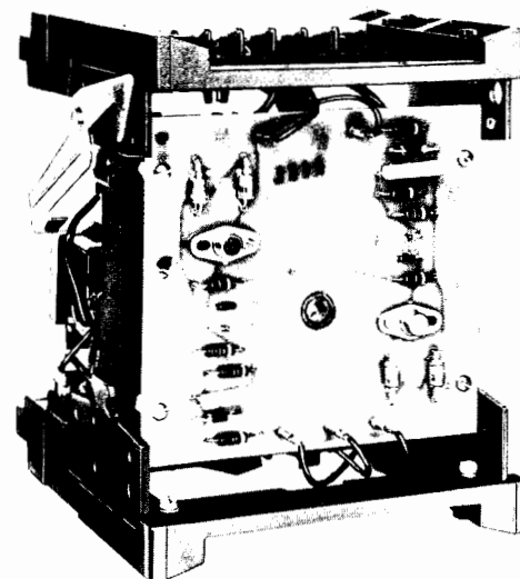
Type ARS Rear View
