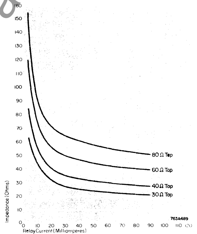
Fig. 9: LC-2 Typical Impedance Curve (impedance is at 22° angle).
