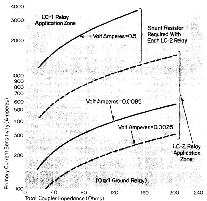
Fig. 3: (Curve C) Approximate phase relay sensitivity (0 or 1 ground relay).
