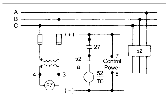
Typical Circuit Shield Undervoltage Relay Application
