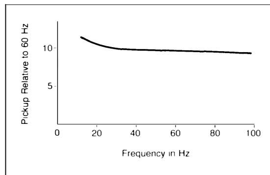
Frequency Response
