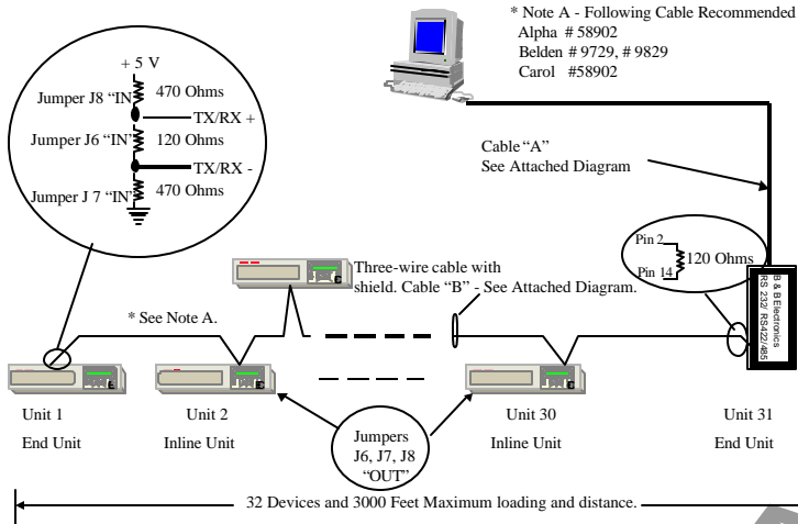
Figure 7 – Termination Using Internal Jumpers And Converter As An End Unit.
