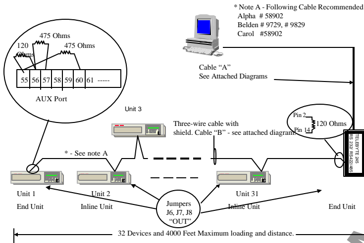
Figure 9 - Termination Using External Resistors On The IED's And Using The B & B Electronics Converter As An End Unit
