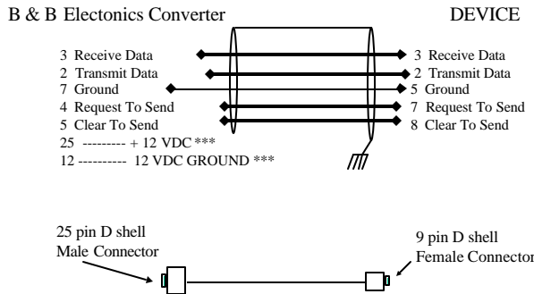
Figure 4 – RS 232 Cable Pinout Handshaking Incorporated (See Figure 1 For Jumper Settings According To Model. DTE To DTE Connection (9 Pin To 25 Pin Rs 232 Converter Connection))
