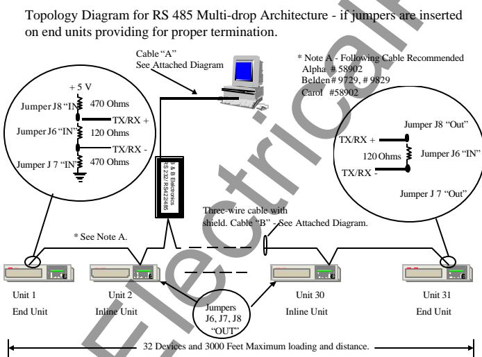
Figure 6 – RS 485 2 Wire Termination With The RS 232/485 Converter Inline And ABB Protective Relays At End Of Line Locations.
