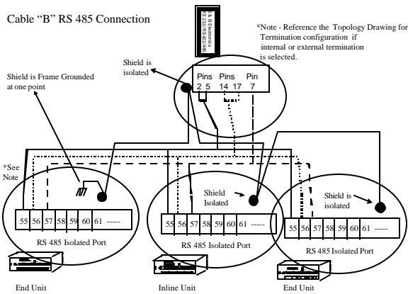
Figure 10 – Conductor Connectivity Diagram For The 2000r Products And The B & B Electronics Converter “Inline”
