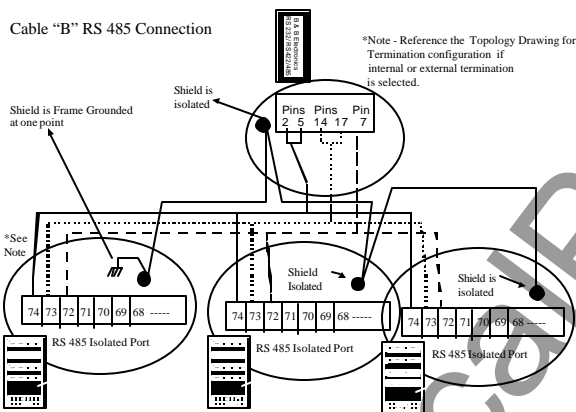
Figure 11 - Conductor Connectivity Diagram For The DPU/TPU 2000 Products
