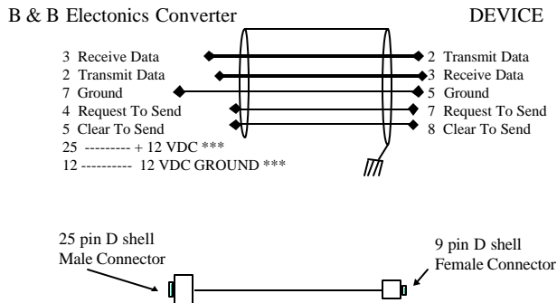
Figure 2 – RS 232 Cable Pinout Handshaking Incorporated (See Figure 1 For Jumper Settings According To Model. DTE To DCE Connection (9 Pin To 25 Pin RS 232 Converter Connection))
