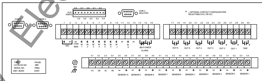
Rear Terminal Blocks and Communication Ports
