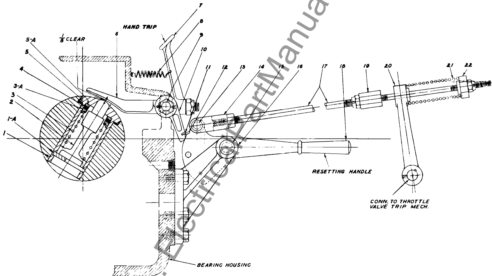
Overpeed Trip Mechanism
