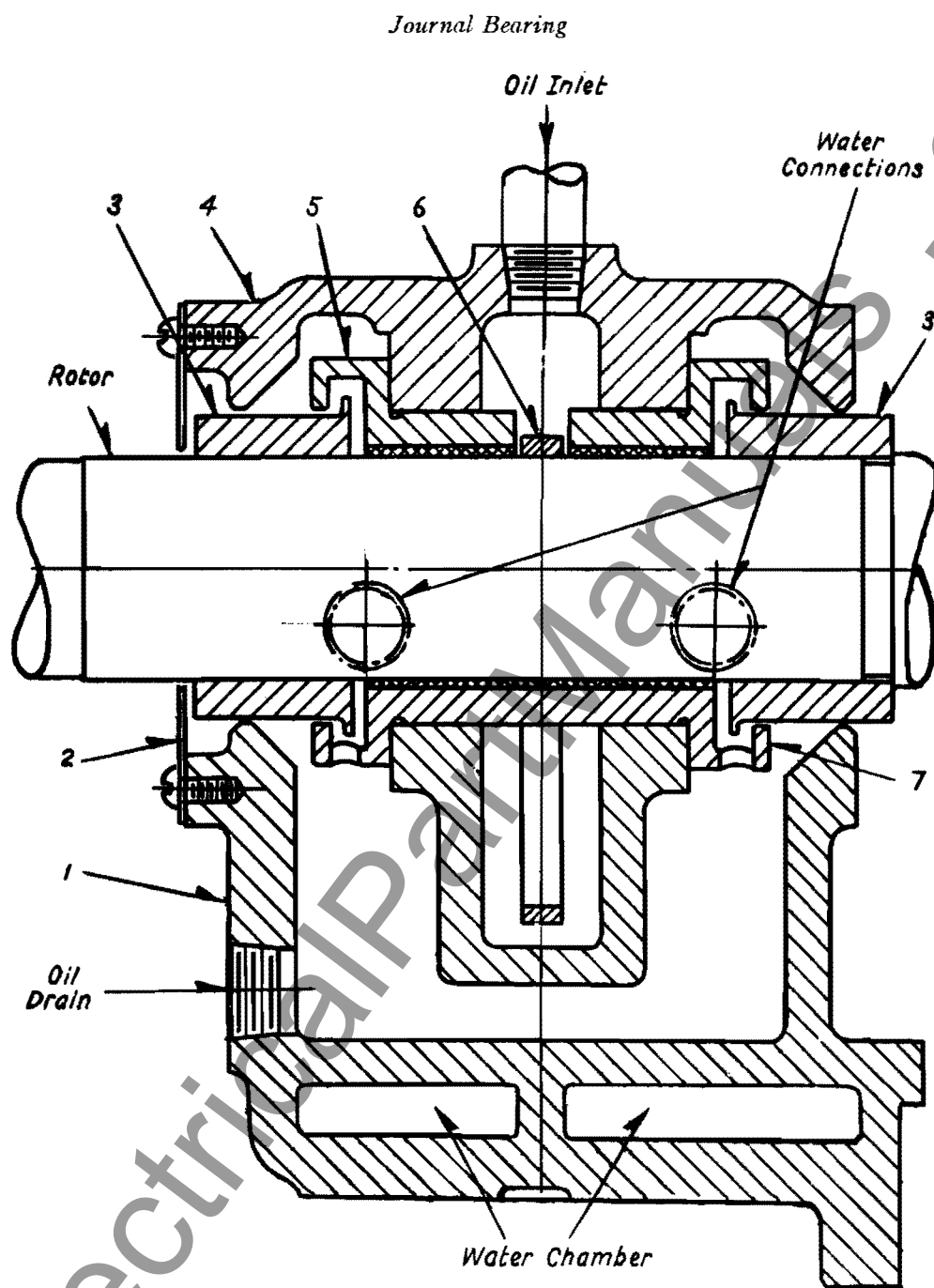
Fig. 1 - Journal Bearing and Bearing Bracket
