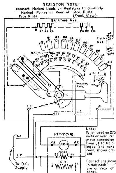
FIG. 5—WIRING DIAGRAM
