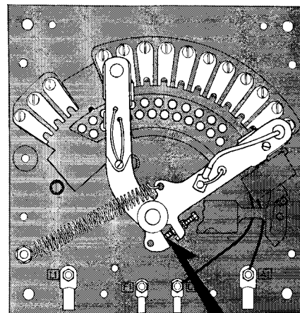
FIG. 3—ON CLASS 7210 RHEOSTATS, A SET SCREW ON THE STARTING ARM CAN BE ADJUSTED TO SET THE MAXIMUM SPEED POSITION OF THE REGULATING ARM.
