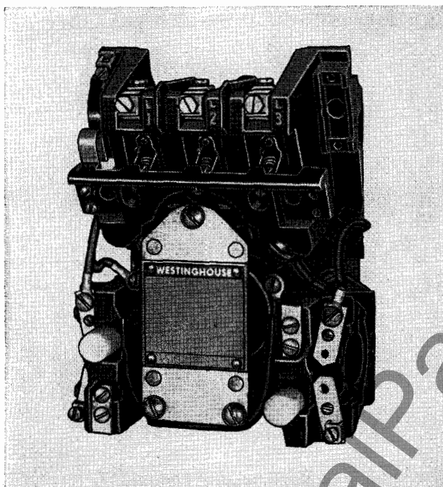
FIG. 1. Size 0, Design N Starter
