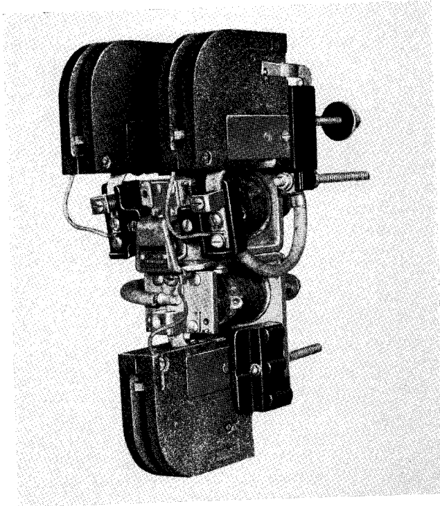
FIG. 1. Types MM-321, 421 Rear-Connected Contactors
