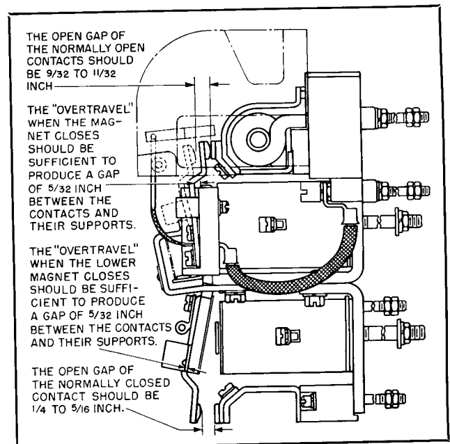
FIG. 2. Sectional View of Types MM-321, 421 Contactors
