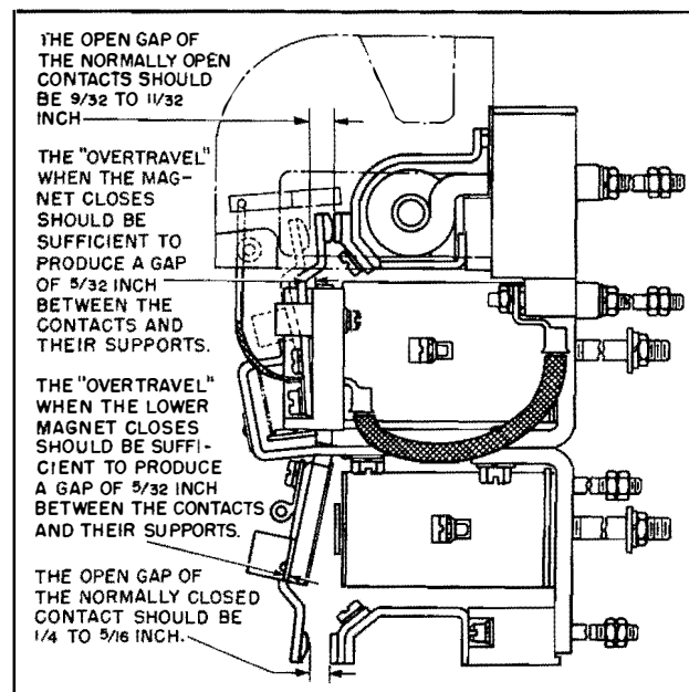
FIG. 2. Sectional View of Type MM-321 Contactor
