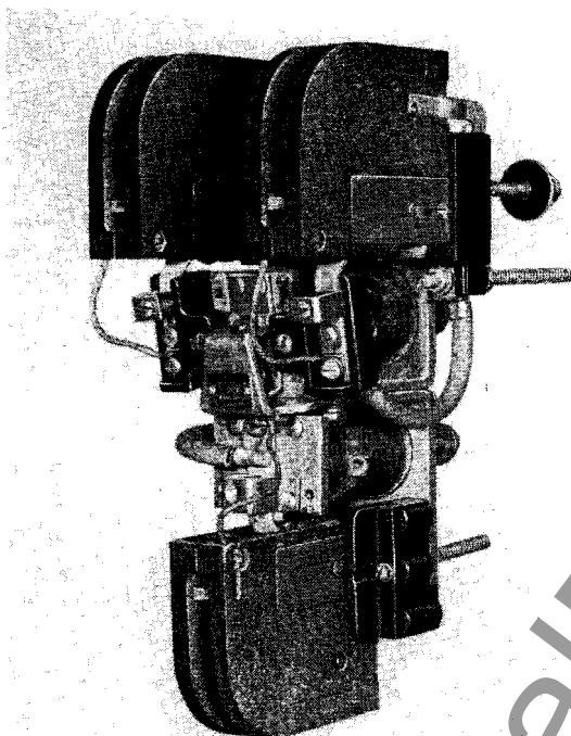
FIG. 1. Type MM-321 Rear-Connected Contactor
