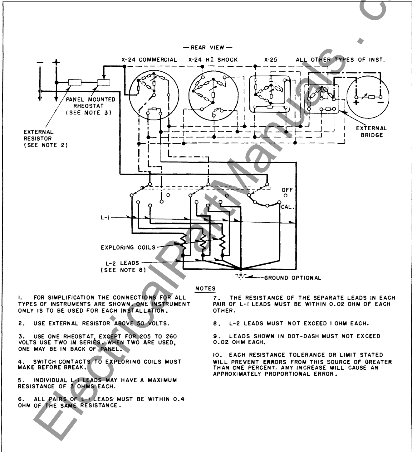
Fig. 8—Exploring Coil Type Temperature Indicator.
