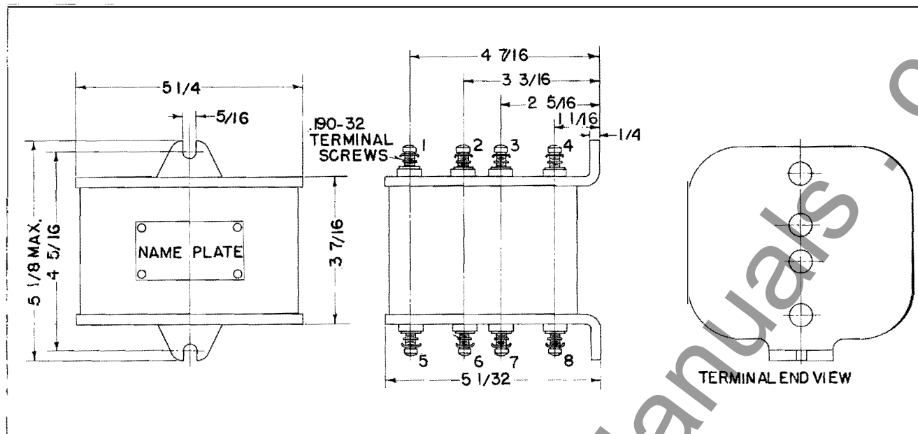
Fig. 4—External Resistor for 205 to 260 Volt d-c Control Voltage. Use Terminal Positions 5 and 6.
