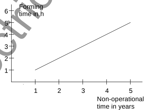
Fig. 6-2 Forming time as a function of the time during which the converter was non-operational
