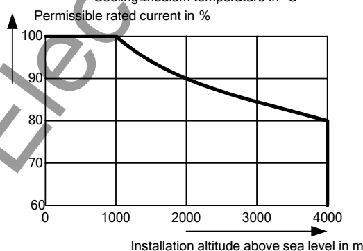
Fig. 11-1 Derating curves
