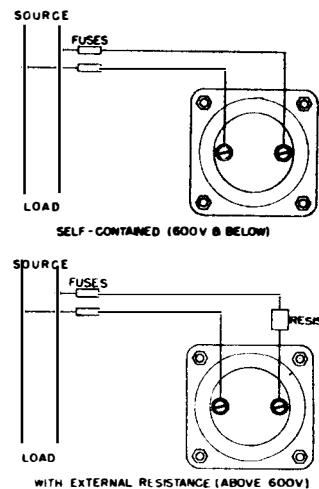
Fig. 7. External connections of a-c voltmeter
