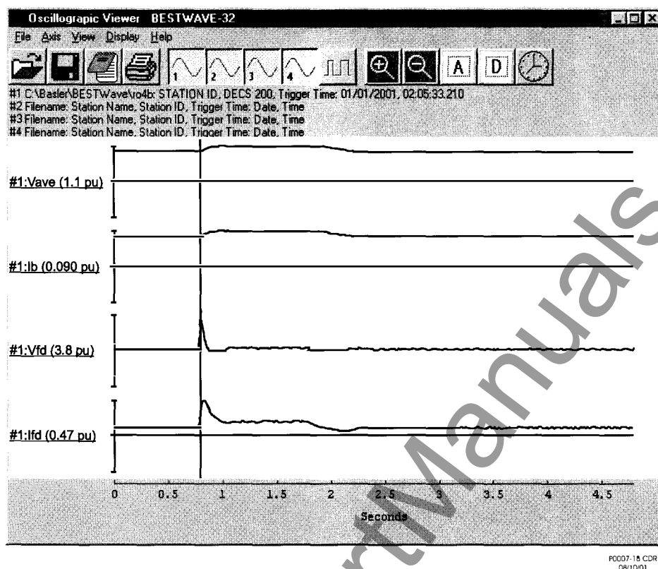
Figure 6 - BESTCOMS Oscillography
