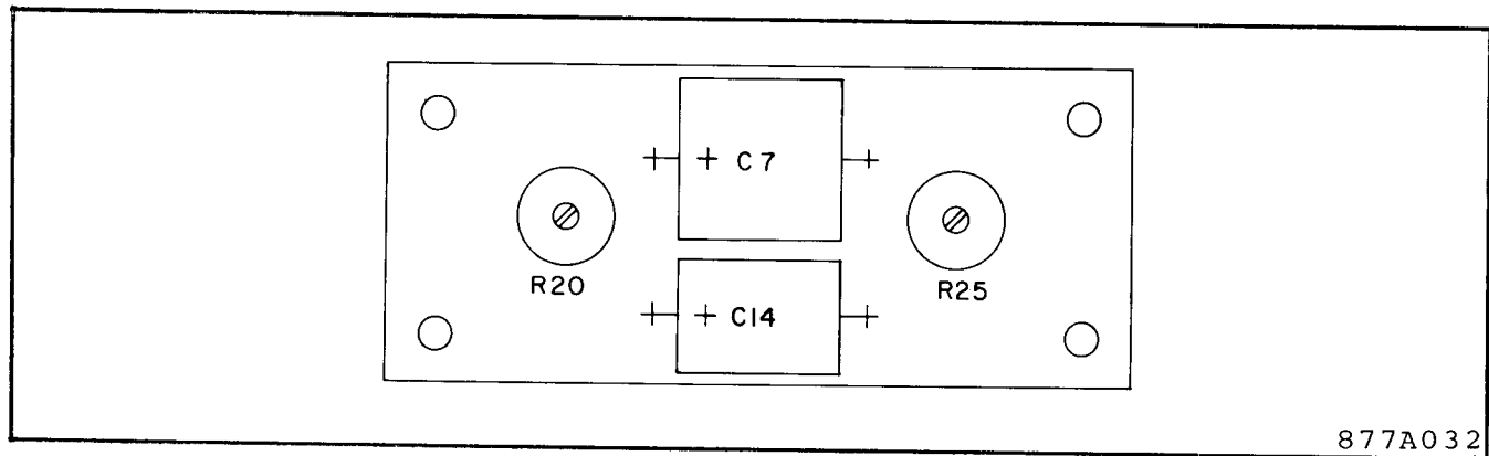
Fig. 6. Component Location (Upper Board)
