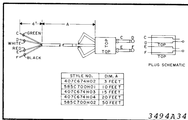
Fig. 4. Patch Cord Assembly
