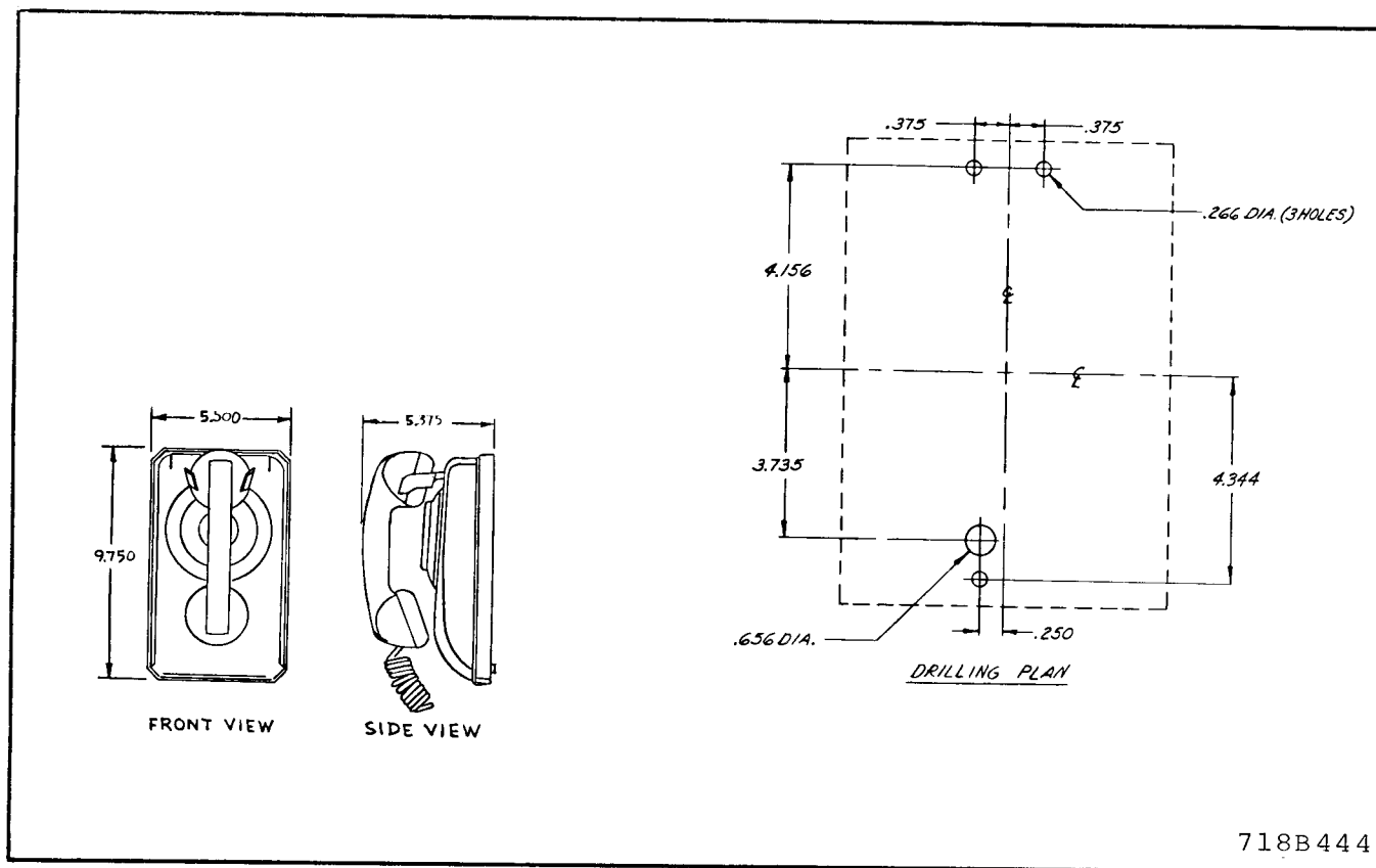
Fig. 10. Mounting Dimensions for Wall Mounted Hookswitch-Handset Assembly
