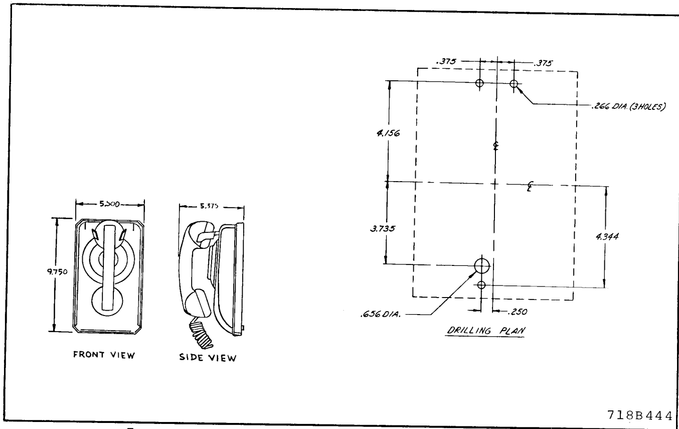
Fig. 10. Mounting Dimensions for Wall Mounted Hookswitch-Handset Assembly
