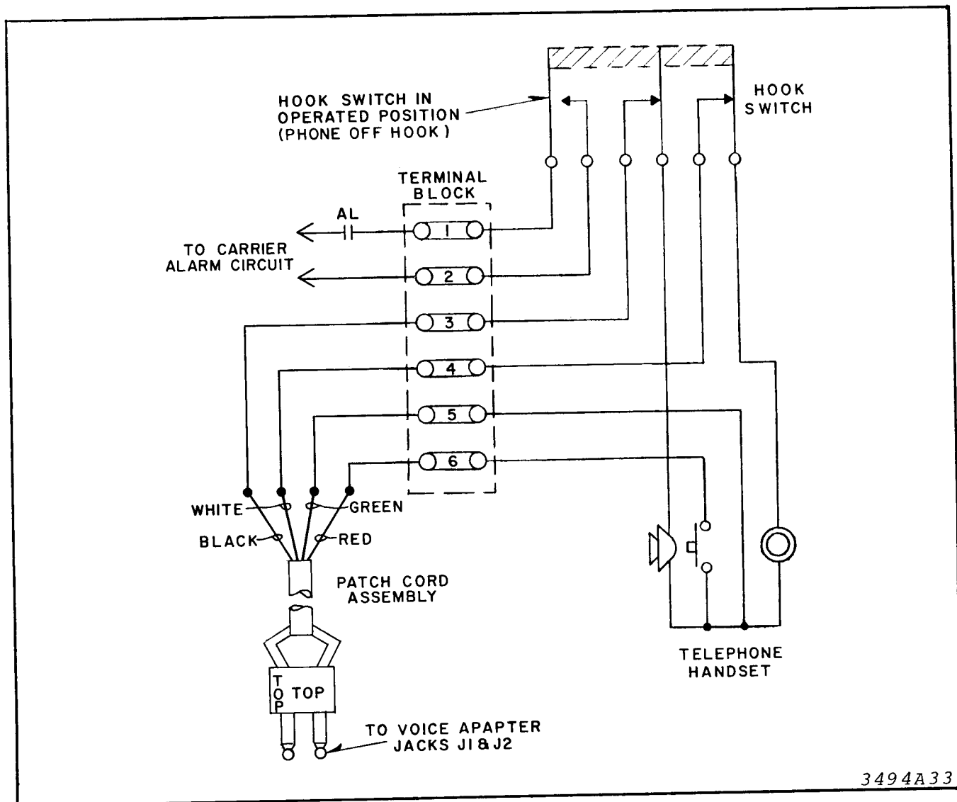
Fig. 12. Telephone Hookswitch - Handset Assembly Internal Schematic and Wiring Diagram.
