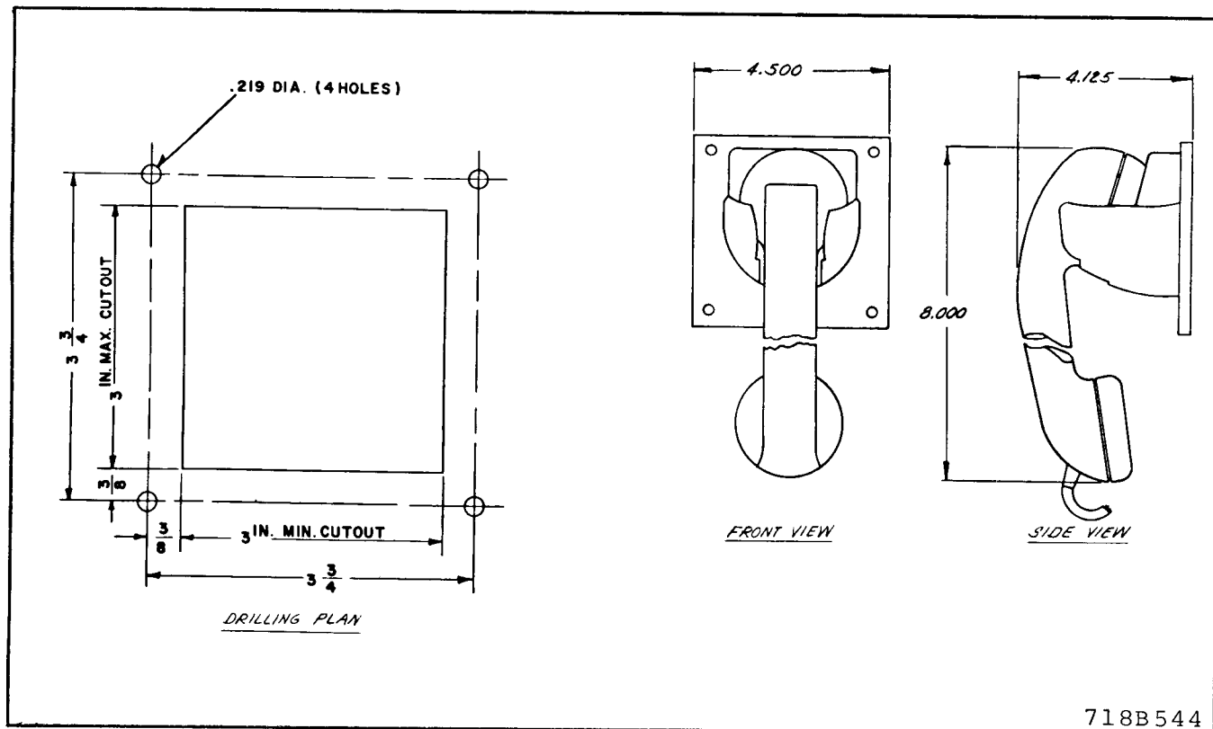
Fig. 11. Mounting Dimensions for Panel Mounted Hookswitch-Handset Assembly
