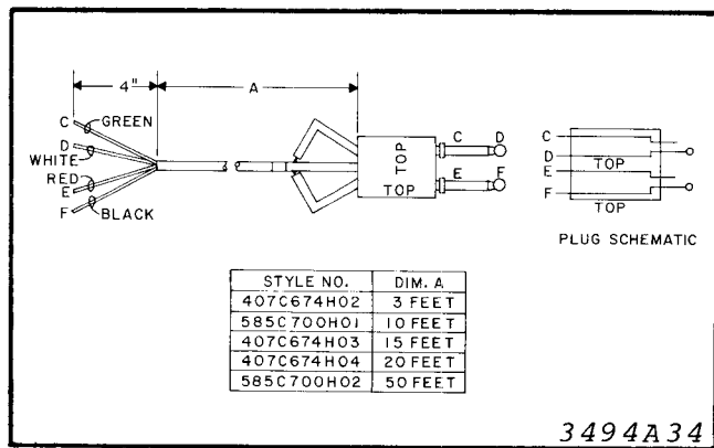
Fig. 4. Patch Cord Assembly
