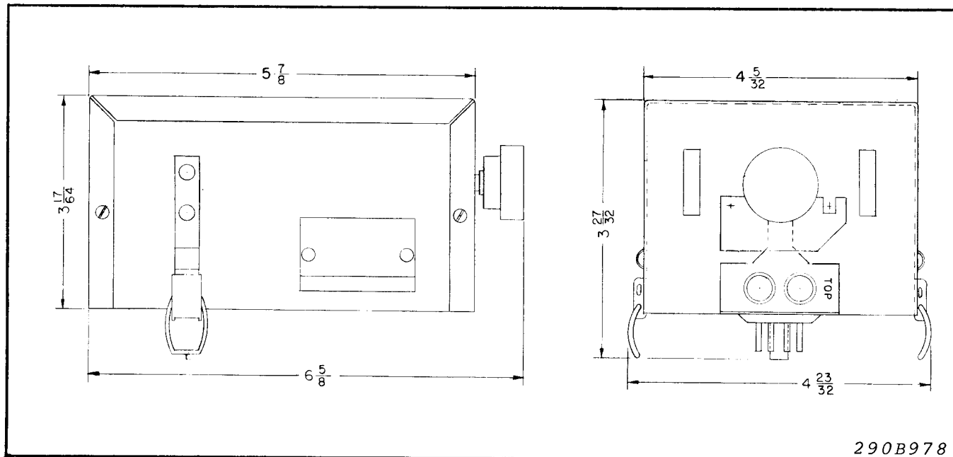
Fig. 2. Outline Dimension
