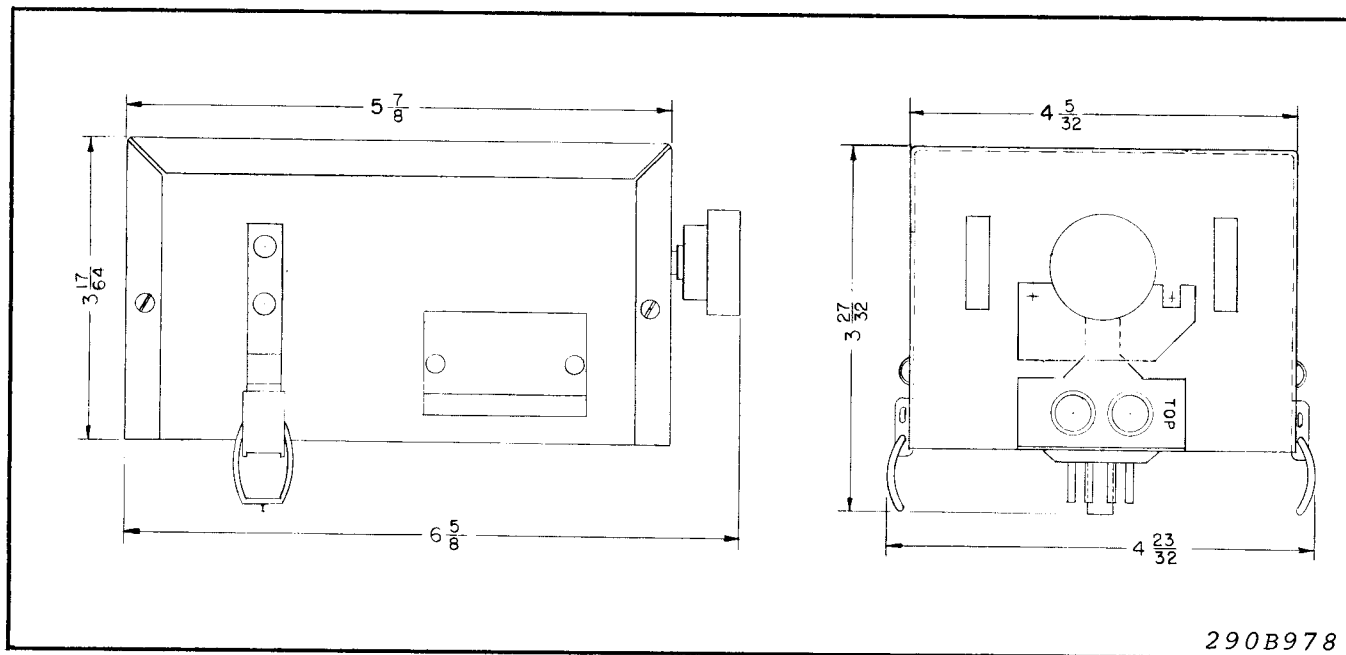
Fig. 2. Outline Dimension
