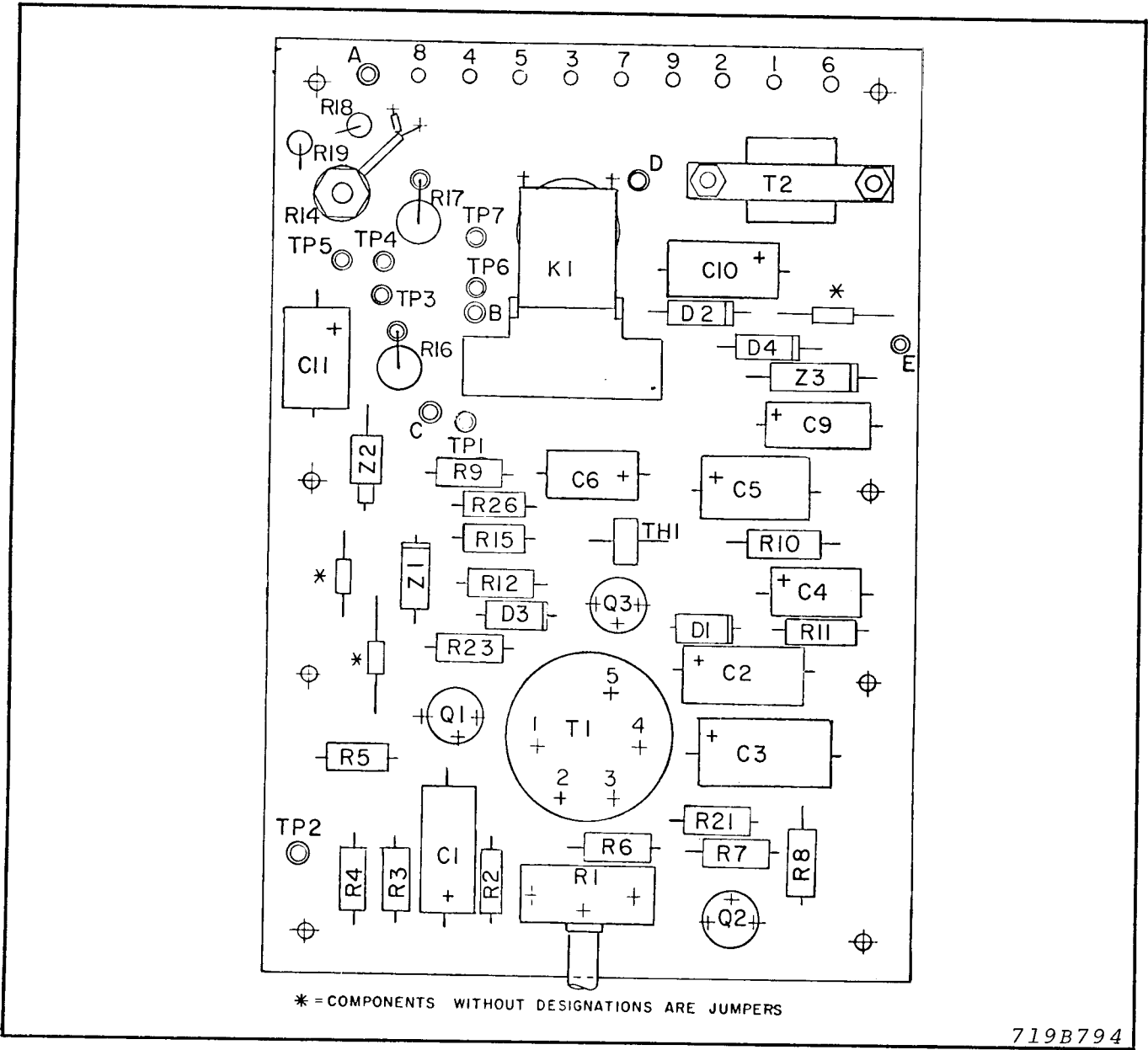
Fig. 7. Component Location (Lower Board)
