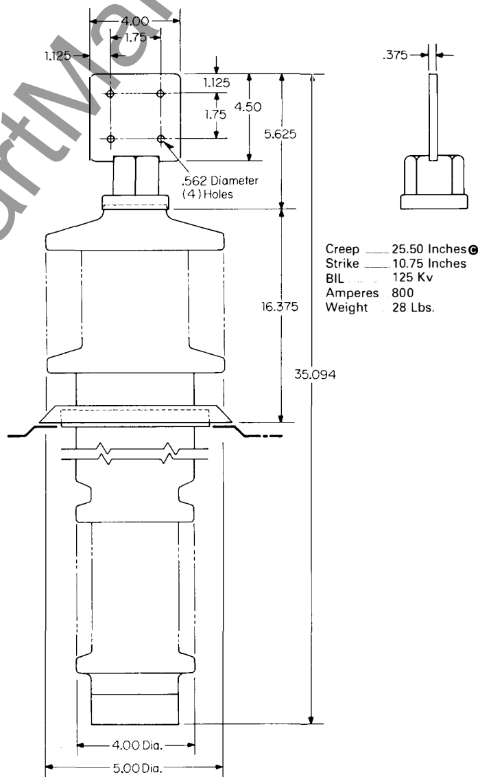
ESV Bushing and NEMA 4 Hole Pad Terminal for 125 Kv BIL
