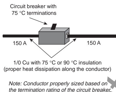
Figure 1: Properly Sized Conductor
