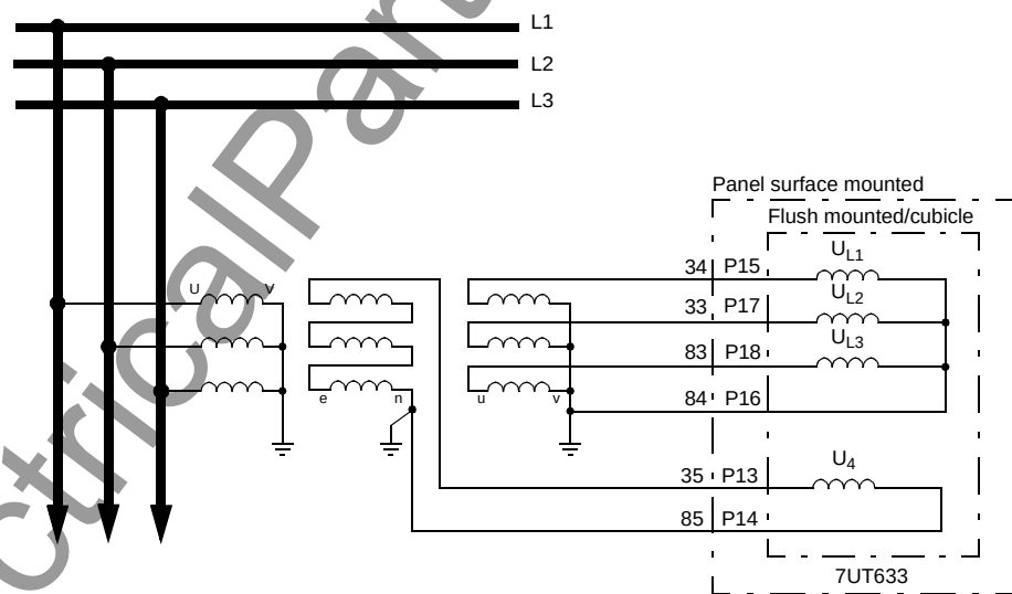
7UT633 (Housing size 1\frac{1}{1} )
