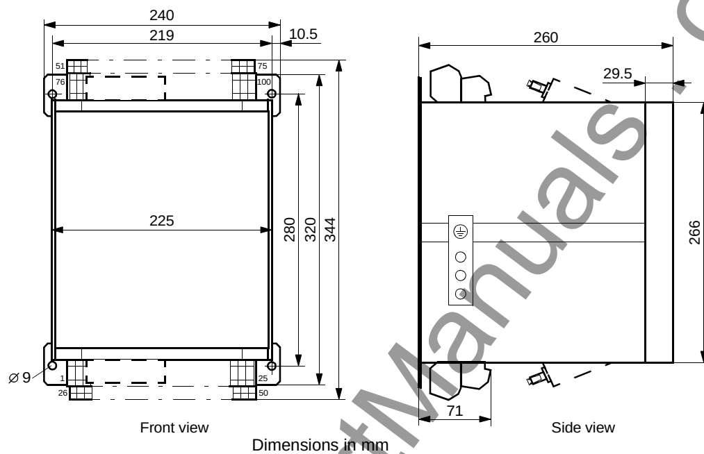
Figure 4-16 Dimensions 7UT613 for panel surface mounting (size 1\frac{1}{2} )
