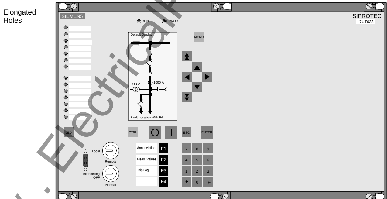
Figure 3-2 Panel mounting of a 7UT633 or 7UT635 with graphic display (housing size 1\frac{1}{2} ) — example
