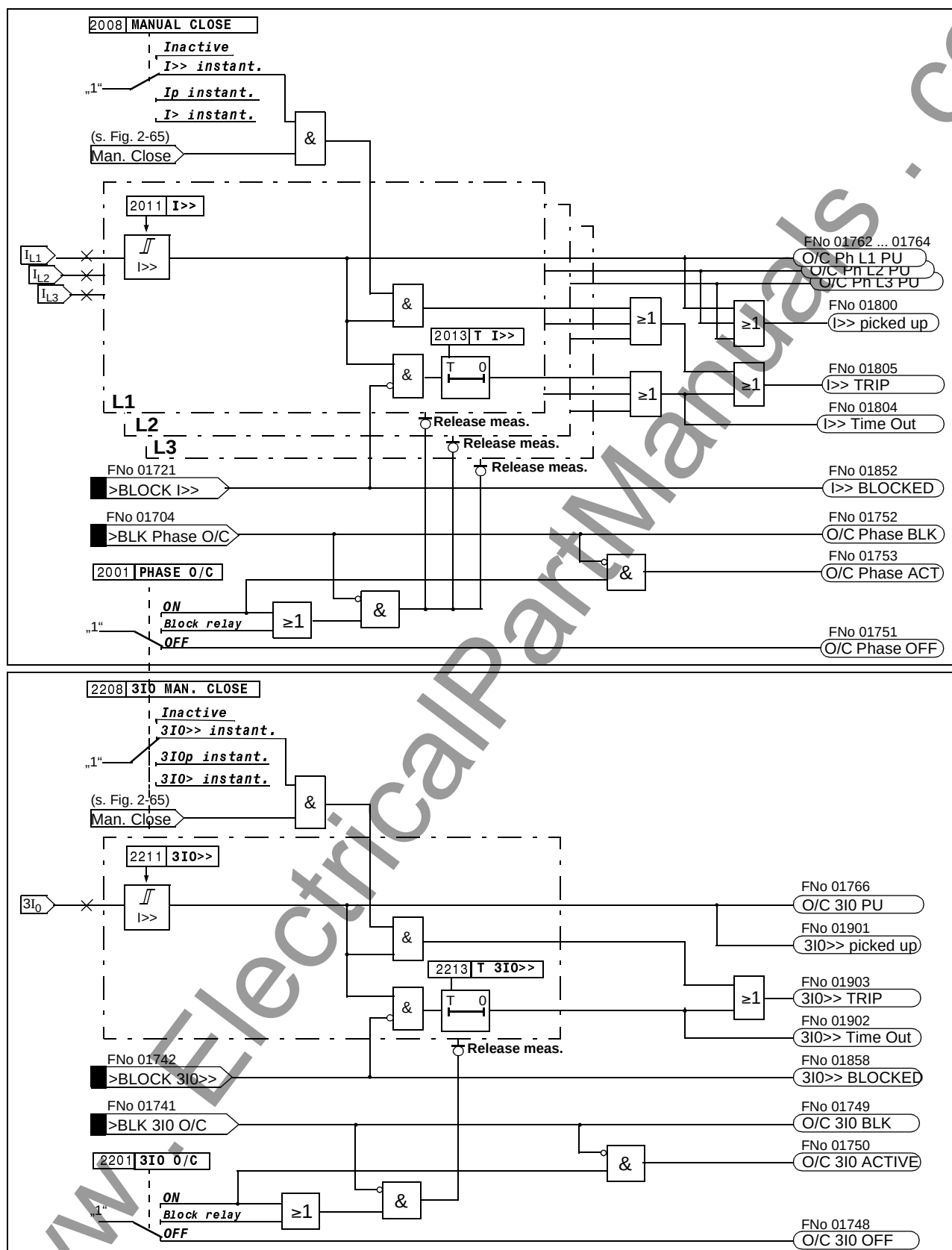
Figure 2-60 Logic diagram of the high-set stages I&gt;&gt; for phase currents and residual current (simplified)
