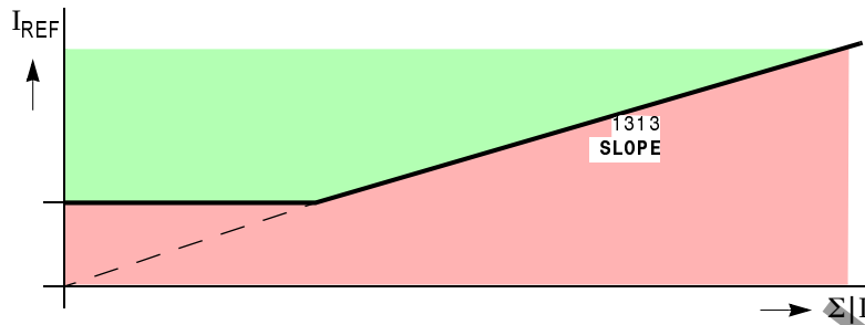
Figure 2-58 Increasing the pickup value
