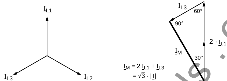
Figure 2-42 Summation of the currents L1-L3-E in the summation transformer
