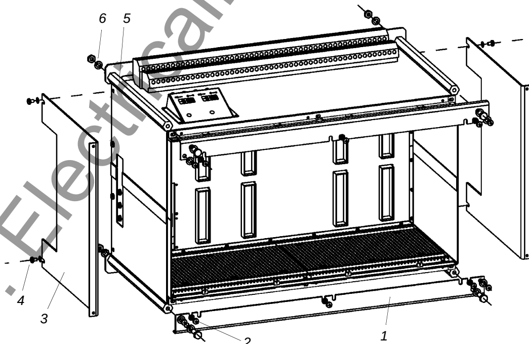
Figure 3-5 View of a housing size 1\frac{1}{1} with transport protection (without front and modules)
