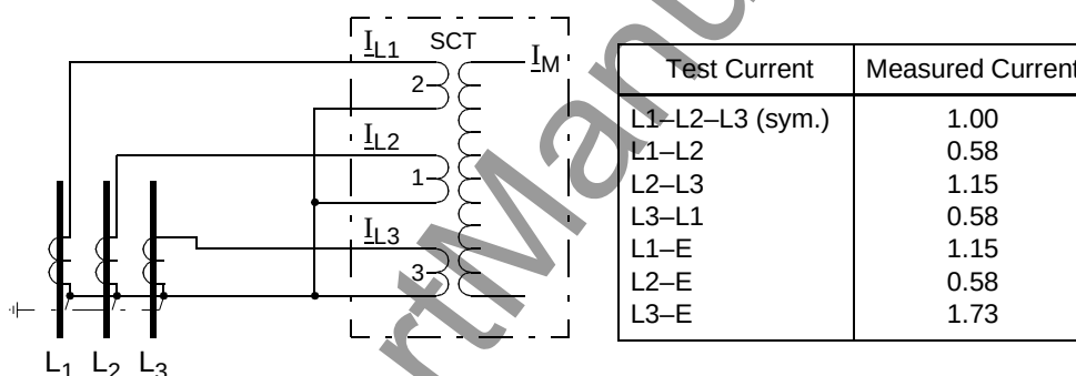
Figure 3-36 CT connection L1-L2-L3
