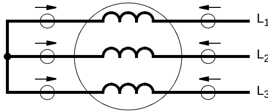
Figure 2-33 Definition of current direction with longitudinal differential protection
