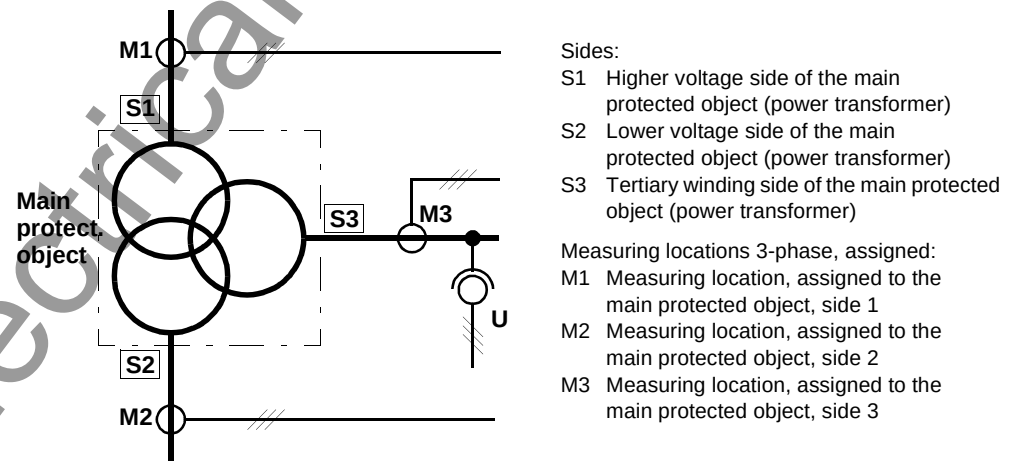
Figure 2-3 Example of a topology on a three-winding transformer
