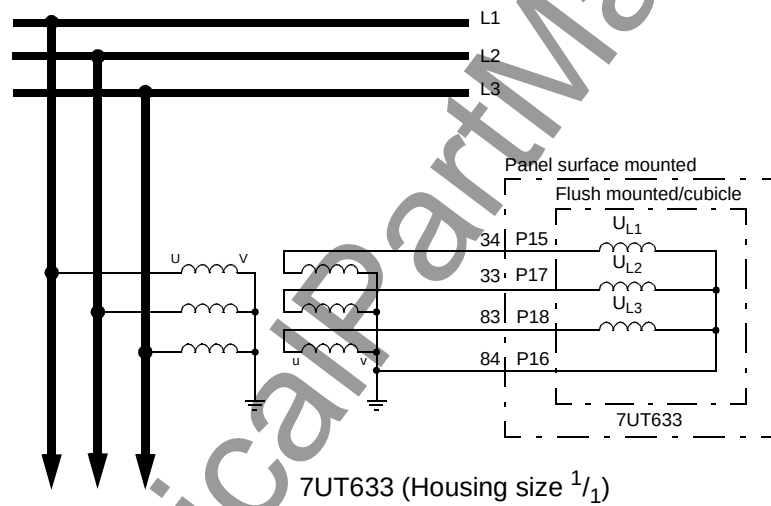
Figure A-26 Voltage transformer connection to 3 star-connected voltage transformers (7UT613 and 7UT633 only)
