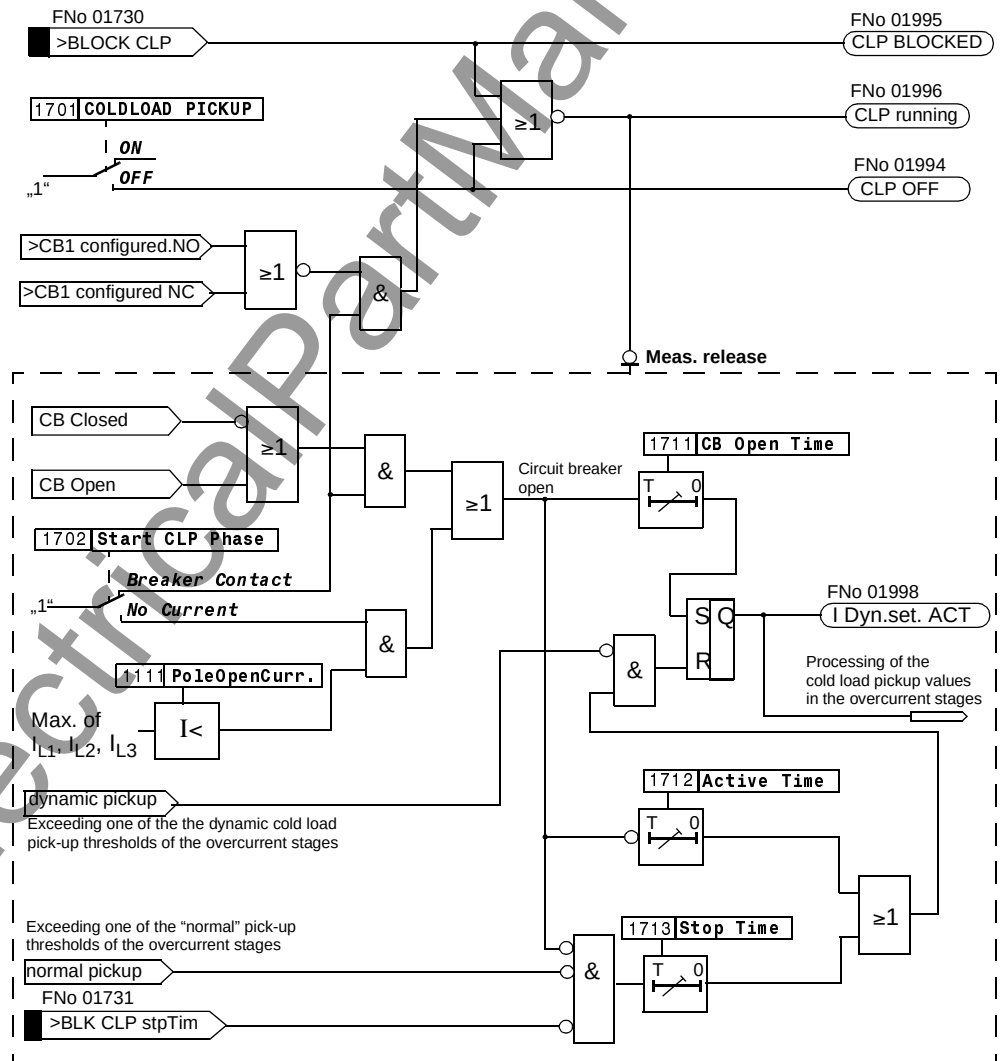
Figure 2-77 Logic diagram for dynamic cold load pickup feature — illustrated for phase overcurrent protection stage on side 1 (simplified)
