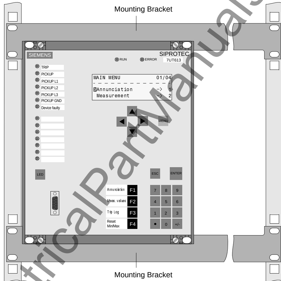
Figure 3-3 Installing a 7UT613 ( 1\frac{1}{2} size housing) in a rack or cubicle — example
