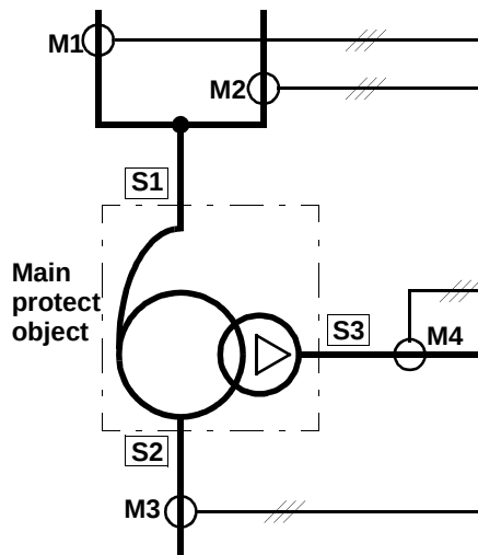
Figure 2-4 Topology of an auto-transformer with a compensation winding which is used as tertiary winding
