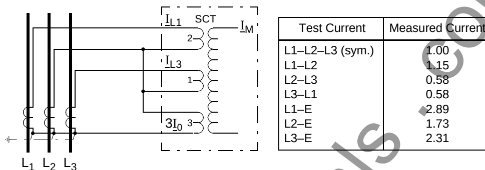
Figure 3-35 CT connection L1-L3-E
