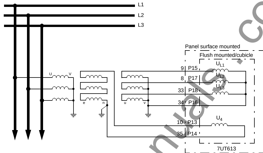
7UT613 (Housing size 1\frac{1}{2} )
