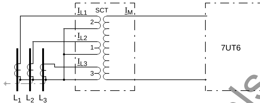
Figure 2-43 CT connection L1-L2-L3 with decreased earth fault sensitivity
