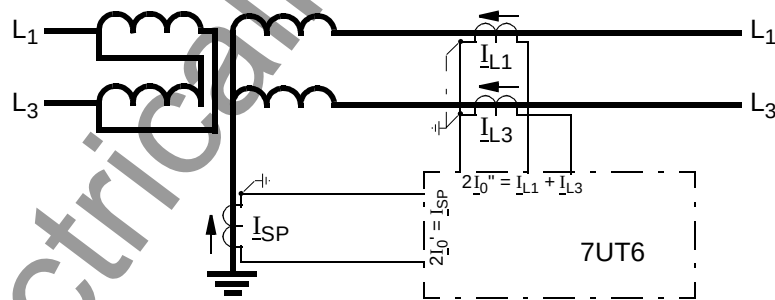
Figure 2-47 Restricted earth fault protection on an earthed winding of a power transformer
