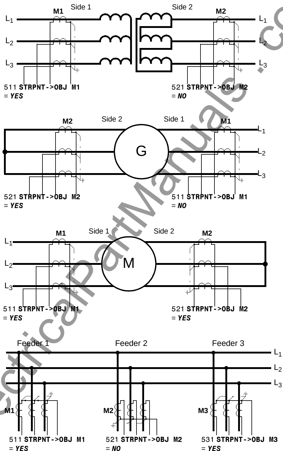
Figure 2-11 Position of the CT starpoints — examples
