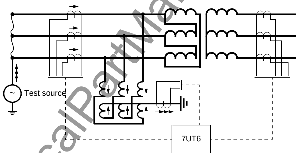
Figure 3-32 Zero sequence current measurement on a delta winding with neutral earthing reactor within the protected zone
