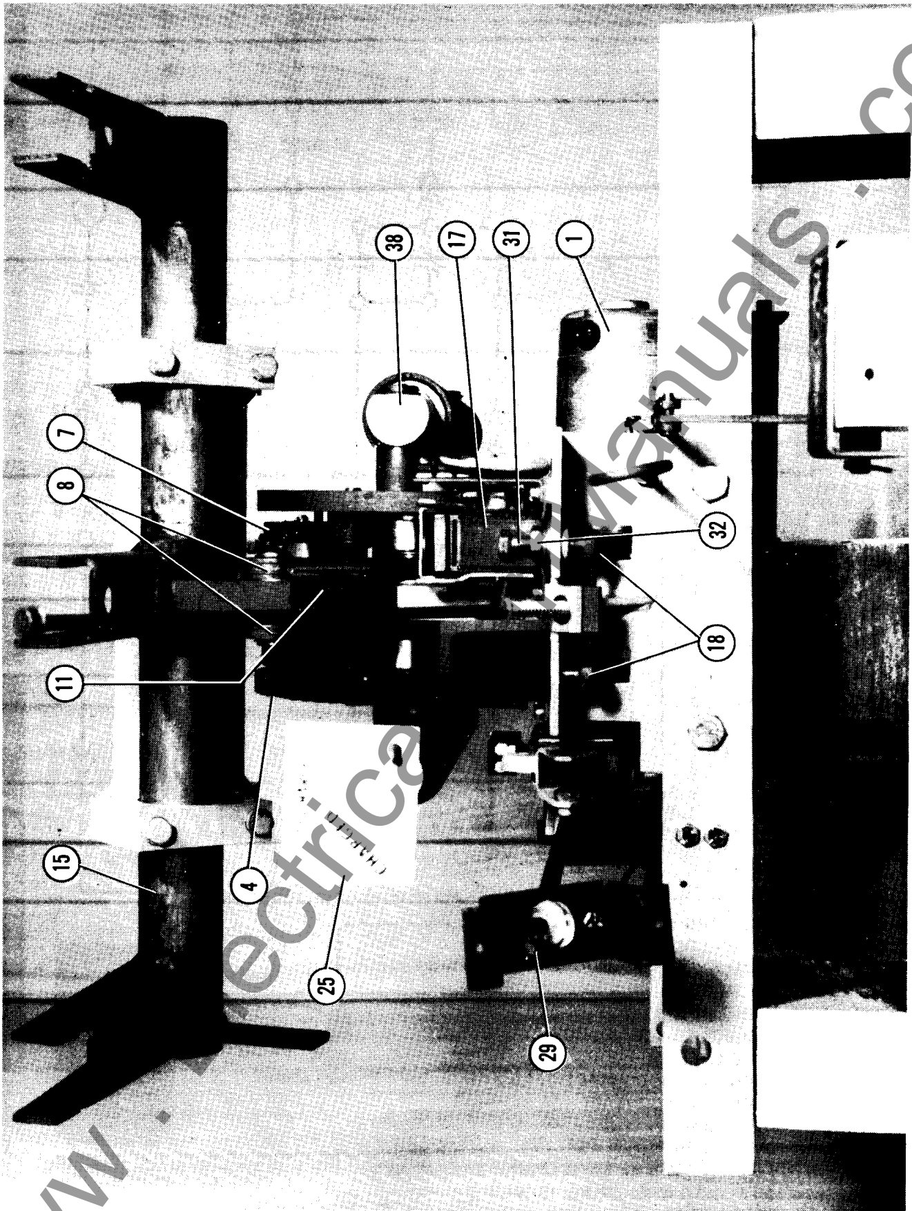
Fig. 11 – 515-2T Operator Front View
