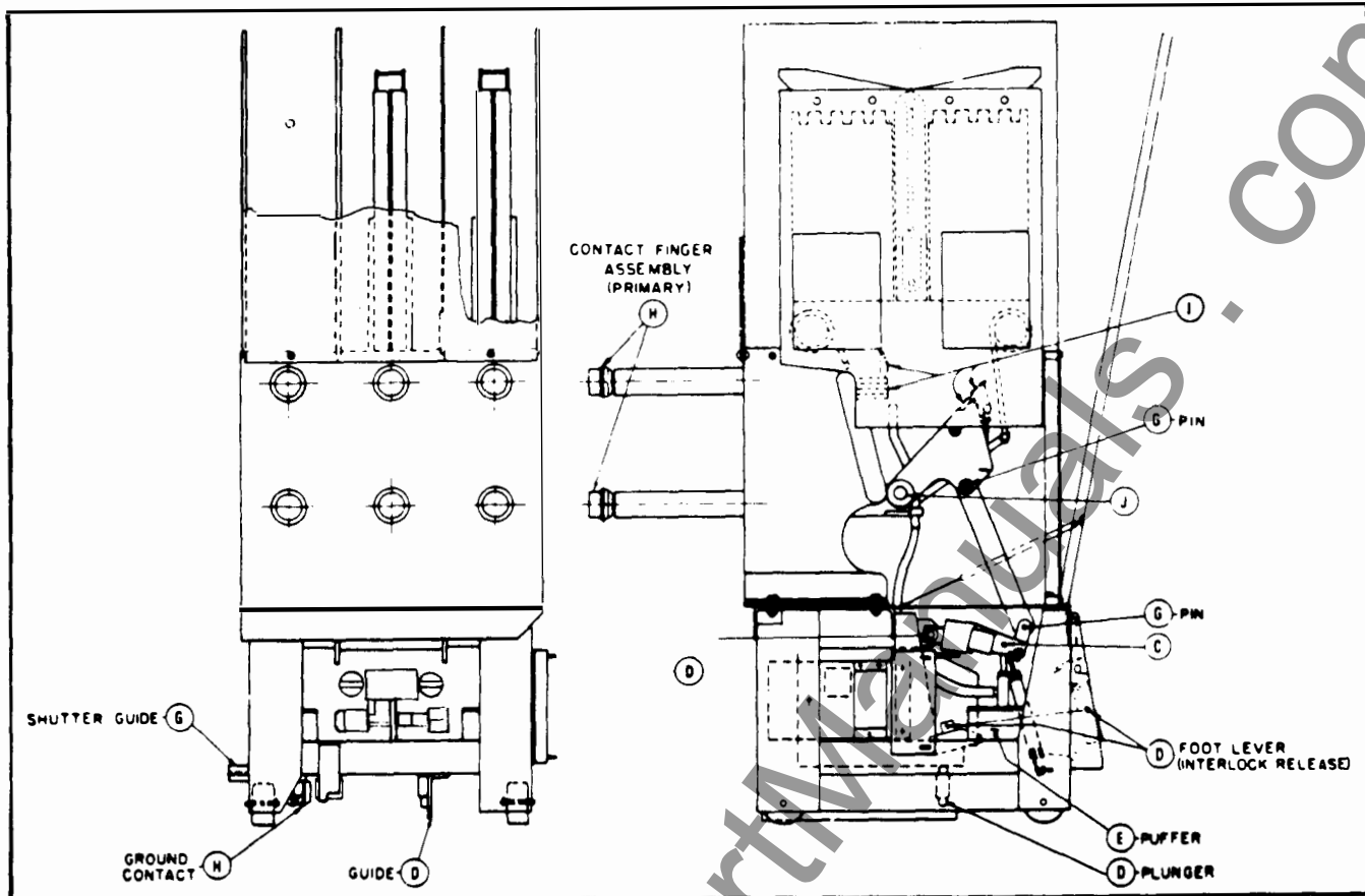
Fig. 20 – Lubrication Points on Breaker
