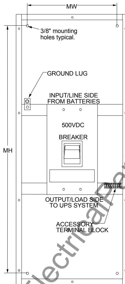
FRONT VIEW COVER REMOVED
