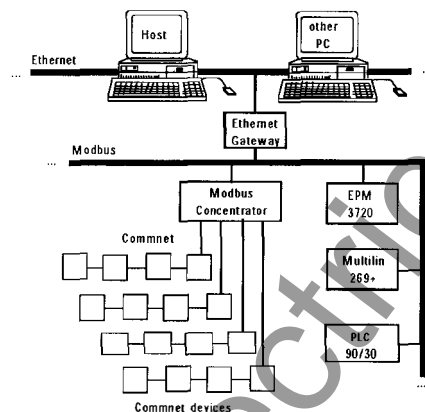
Figure 4. Ethernet, Modbus, and commnet network.
