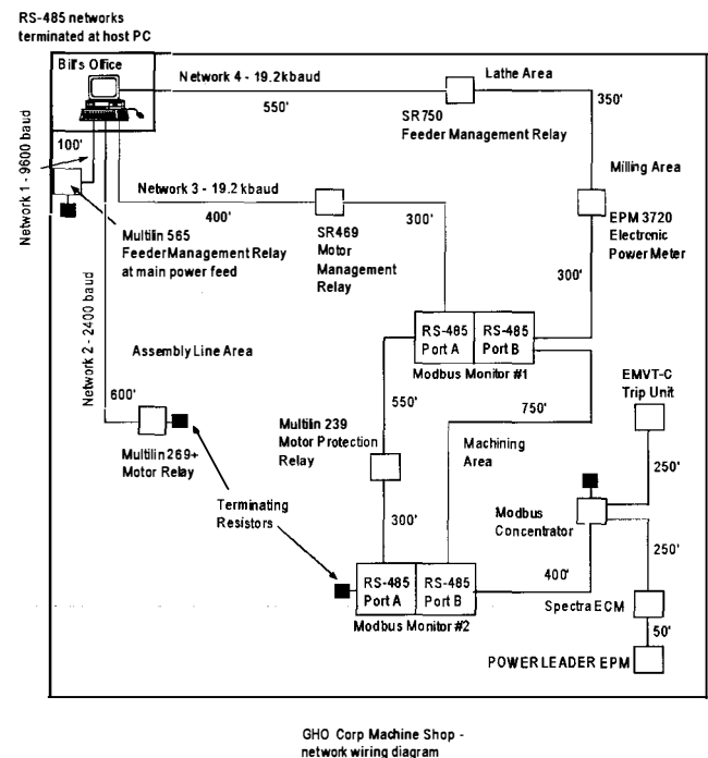
Figure 27. Floor layout for Case Five.
