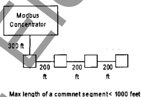
Figure 16. Network illustrating commnet Rule 2.
