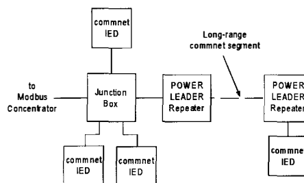
Figure 20. Network illustrating commnet Rule 6.
