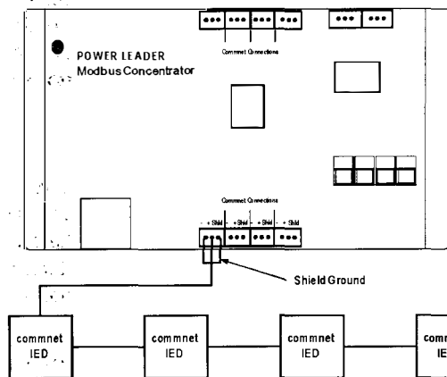
Figure 28. Commnet shield grounding wired correctly.
