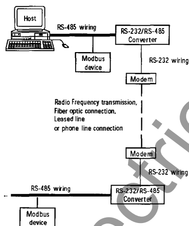
Figure 6. Example of remote operation using modems.
