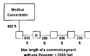
Figure 17. Network illustrating commnet Rule 3.
