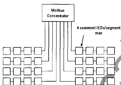
Figure 15. Network illustrating commnet Rule 1.
