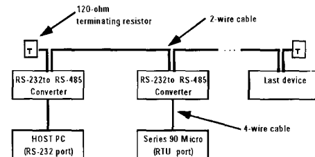
Figure C-1. RS-485 two-wire Modbus network.
