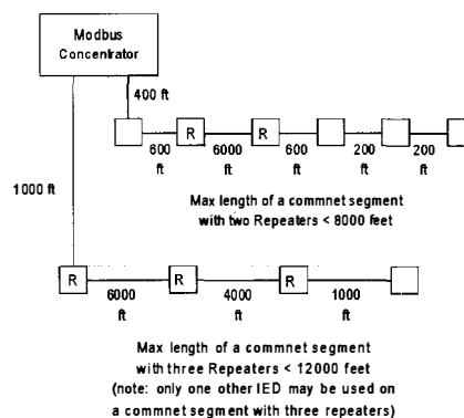
Figure 18. Network illustrating commnet Rule 4.
