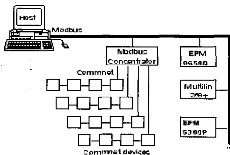
Figure 3. Modbus and commnet network.
