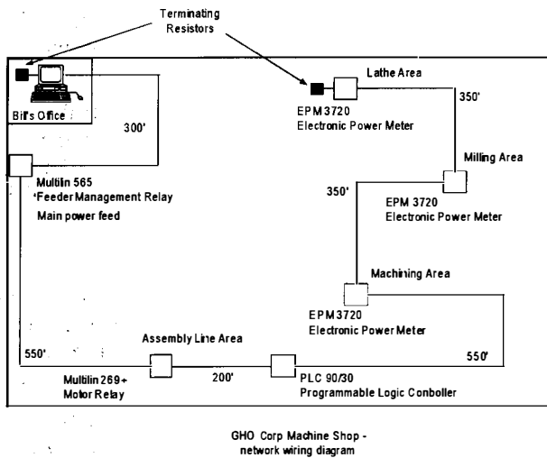
Figure 22. Floor layout for Case One.
