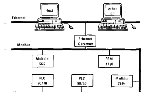
Figure 2. Commercial Ethernet and Modbus network.
