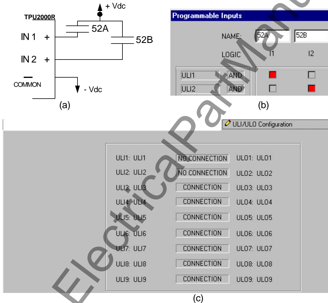
Figure 6 - TPU2000R Breaker Monitoring: (a) typical connections; (b) programmable input mapping; (c) ULI/ULO configuration.
