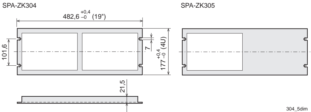
Fig. 4 Mounting cabinets and frames (dimensions in mm)
